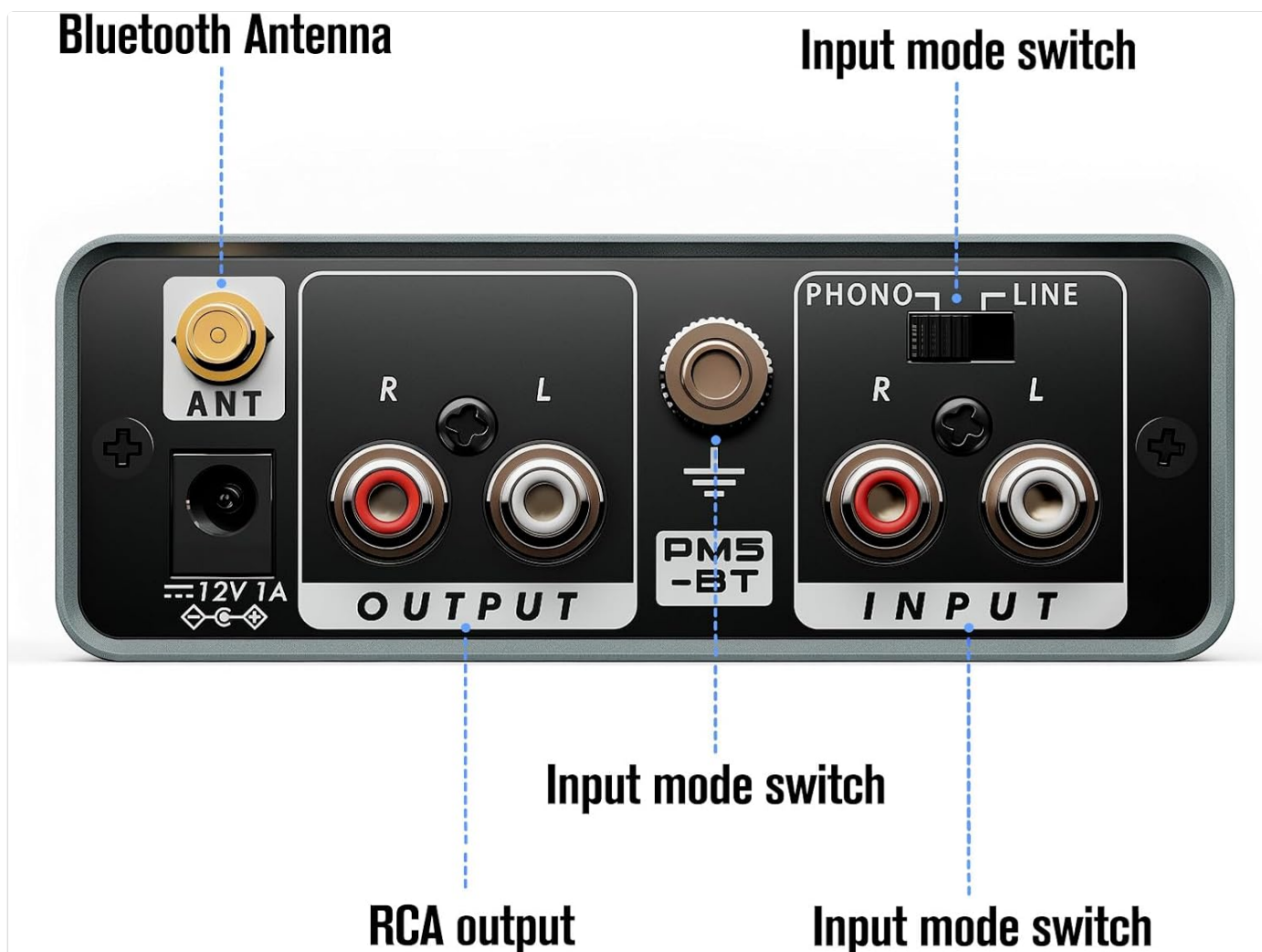
Figure 3: Rear Panel of the PM5BT Preamp
