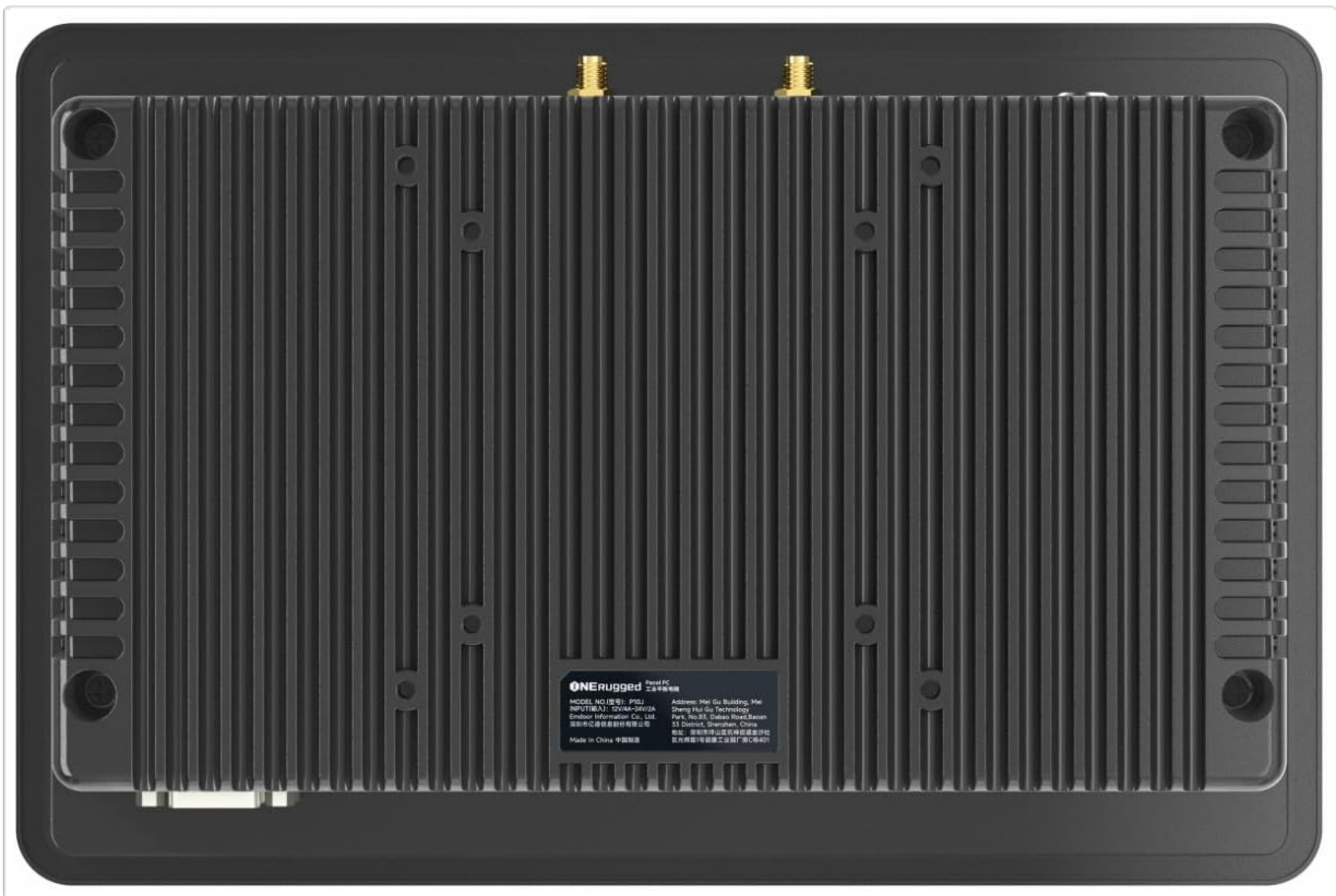
Figure 3.2: Rear view of the ONERugged P10J, highlighting the fanless design with heat dissipation fins and various port labels.
