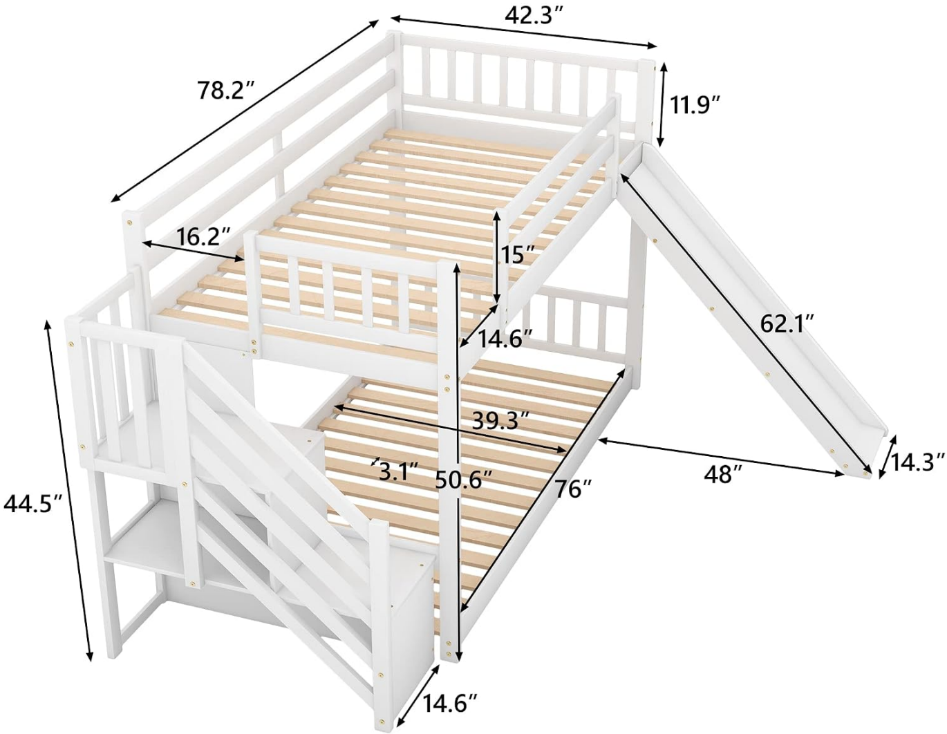
Image 5: A technical diagram showing the precise dimensions of the LUMISOL Twin Over Twin Bunk Bed in inches, including length, width, height, and individual component measurements like the slide and stairs.
