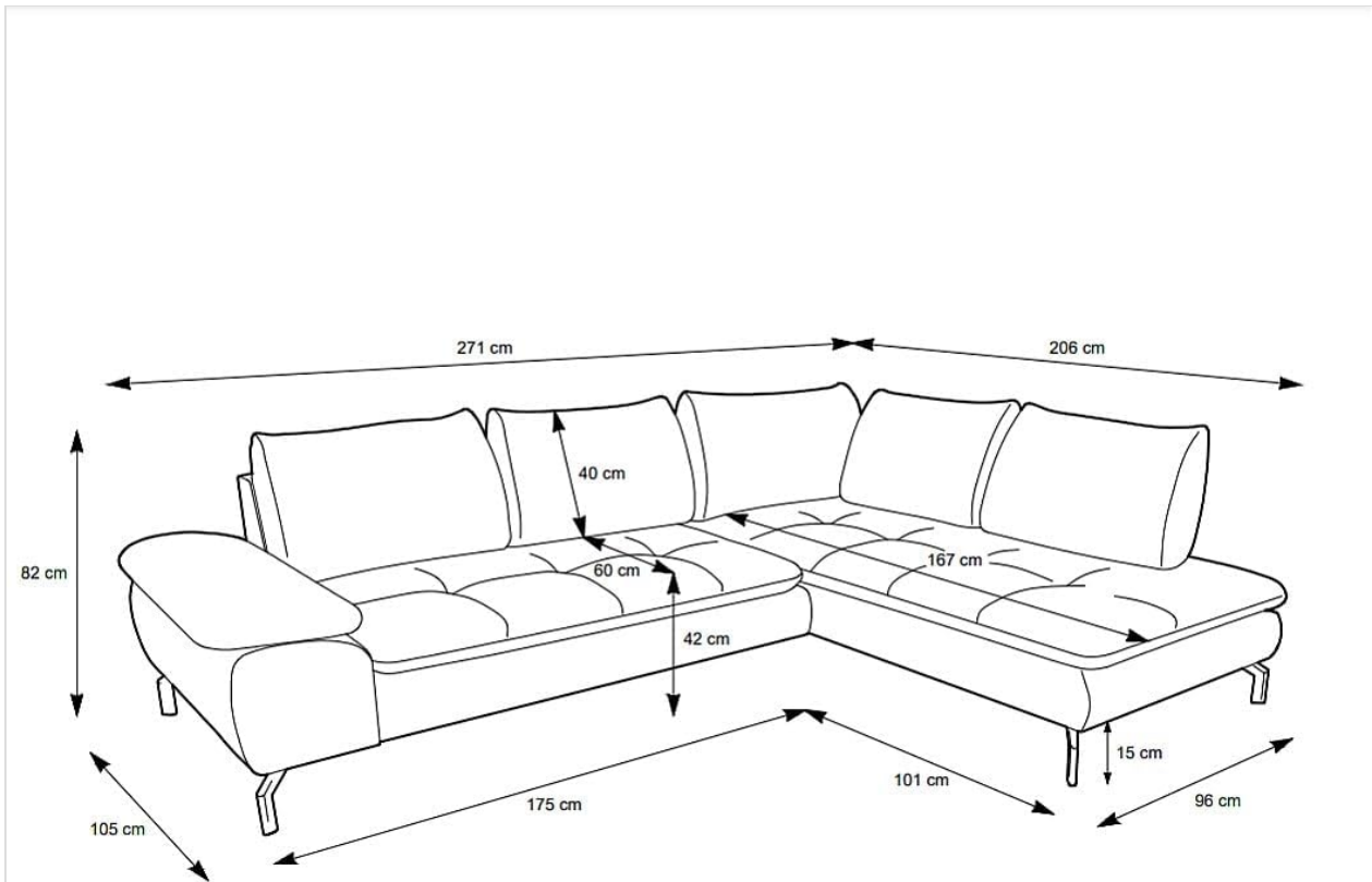
Image 3.1: Dimensional diagram of the Archibald sofa.
