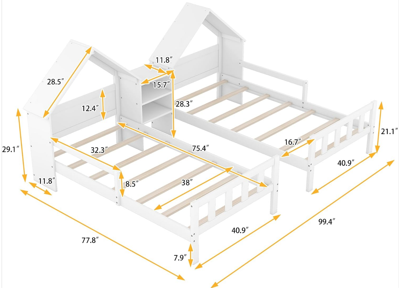
Image 5: Technical diagram illustrating the precise dimensions of the LUMISOL Double Twin Bed Frames in inches.
