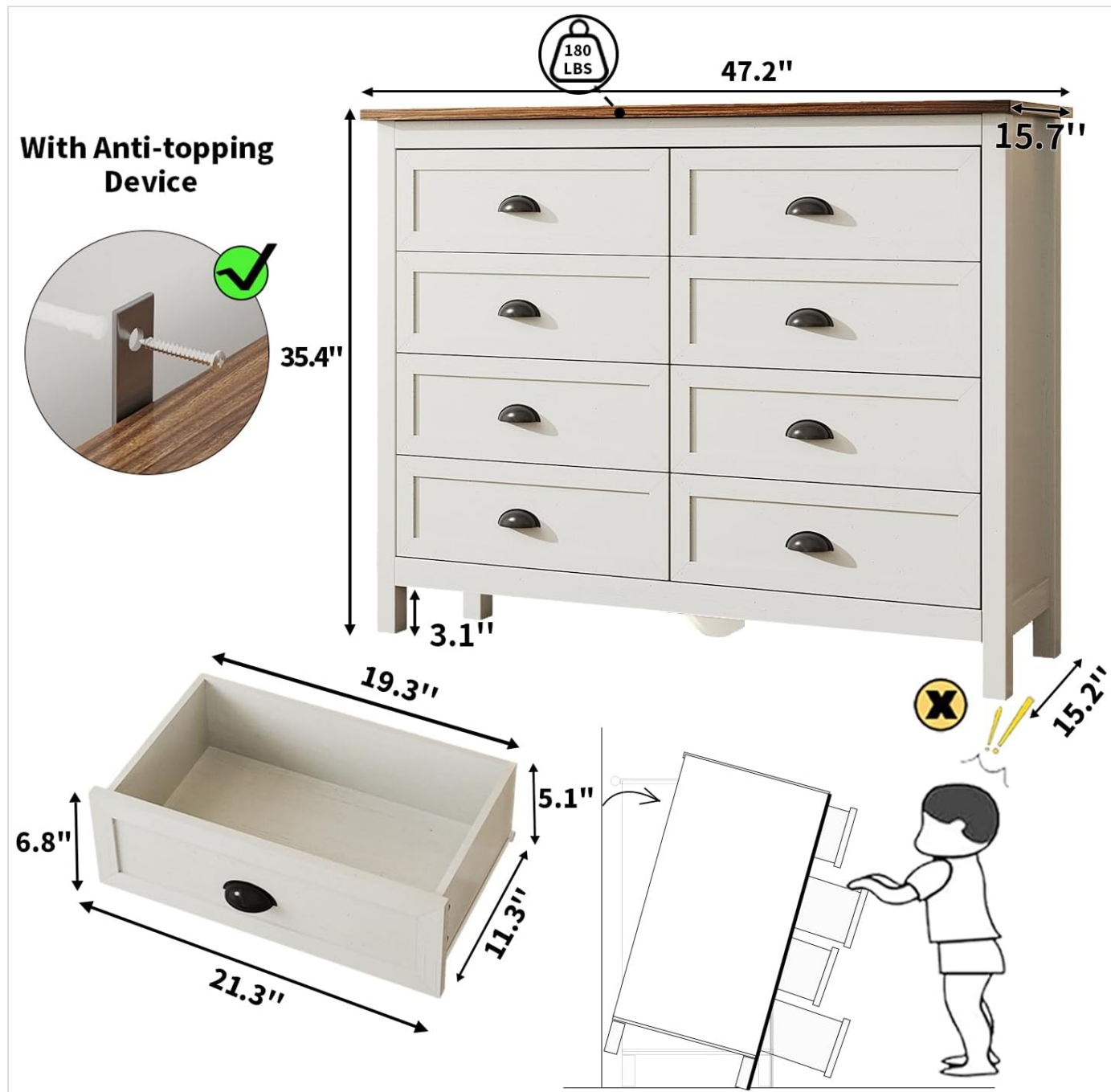
Figure 2: This diagram illustrates the key dimensions of the dresser and highlights the anti-tipping device, emphasizing safety and stability.
