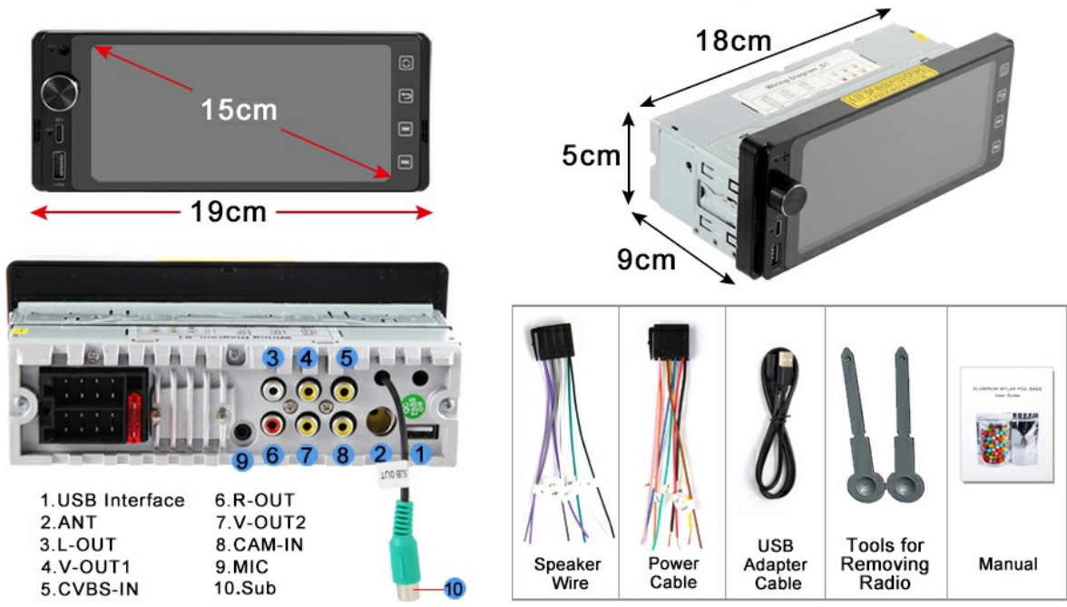
Image: Wiring diagram and connection points.
