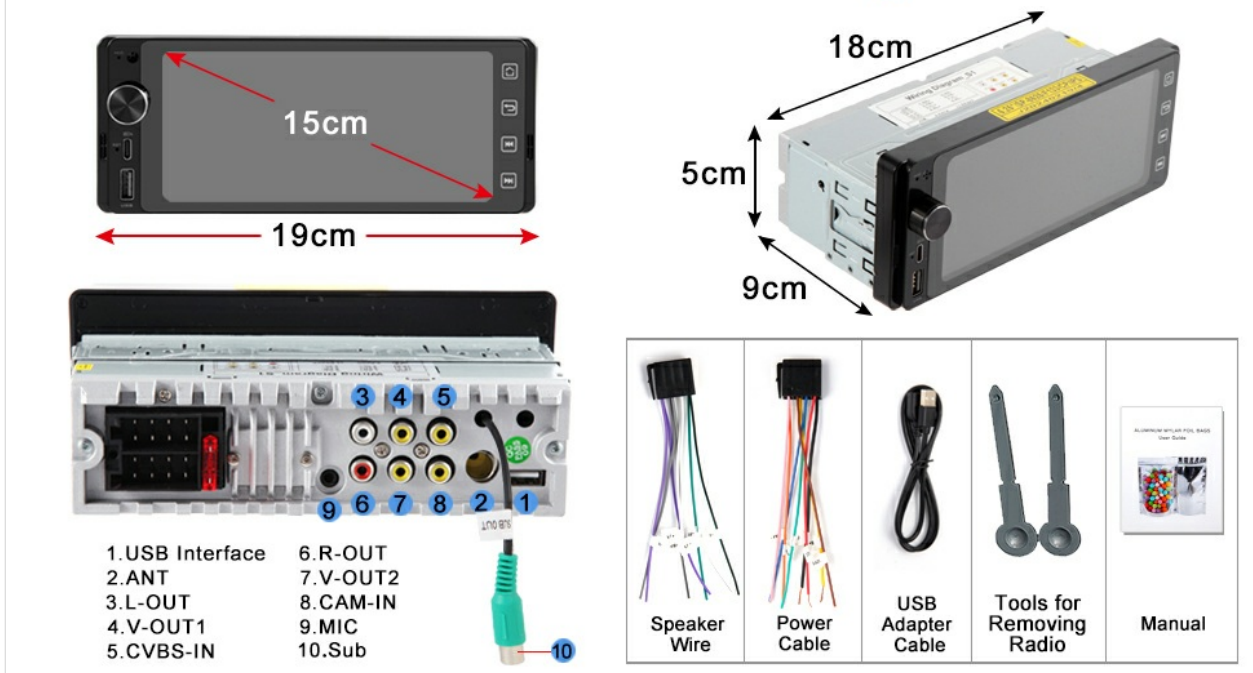
Image: Product dimensions and included accessories.
