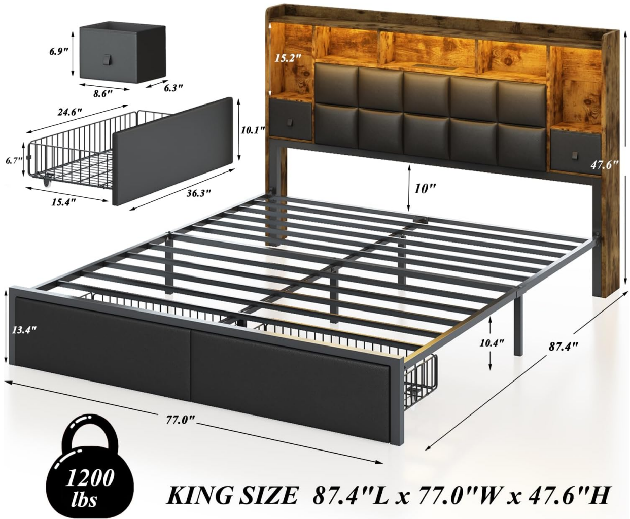
Image: Detailed diagram illustrating the dimensions of the King Size LED Bed Frame.
