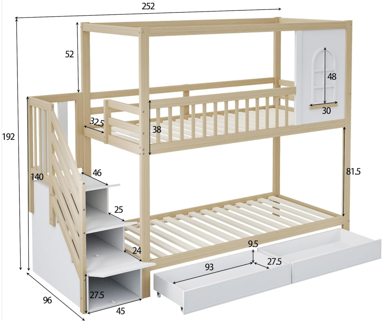
Image 1: Detailed dimensions of the Moimhear Bunk Bed. This image illustrates the overall length (252 cm), width (96 cm), and height (192 cm) of the bunk bed. It also provides specific measurements for the ladder steps, the height between bunks, and the dimensions of the storage drawers, crucial for assembly and space planning.
