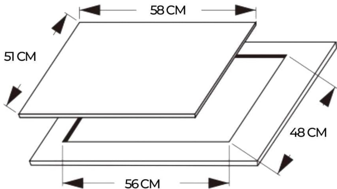
Image: A technical drawing indicating the required countertop cut-out dimensions for installation: 56 cm in width and 48 cm in depth.
