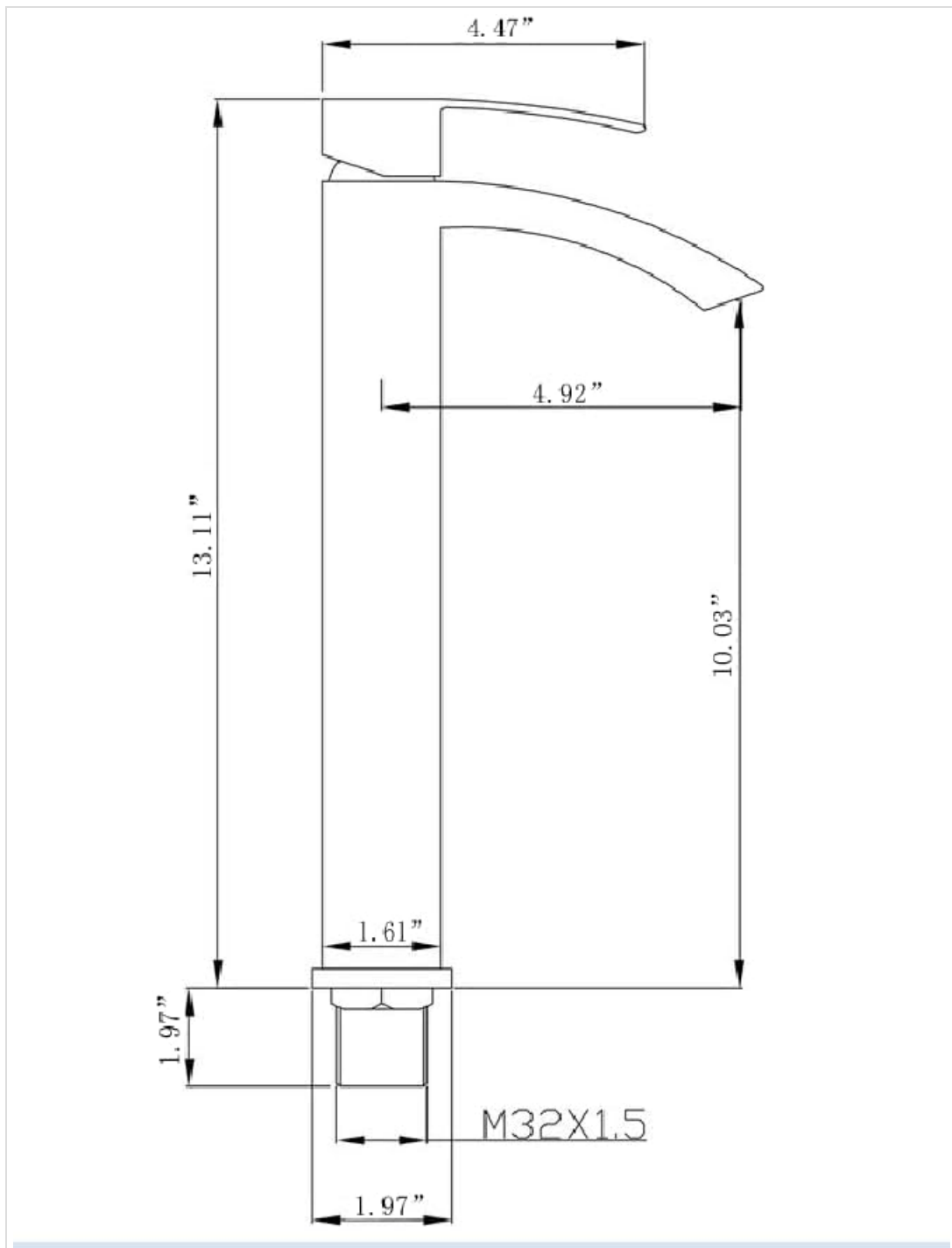
Figure 1: Technical diagram showing the dimensions of the WELLFOR NK Faucet, including spout height (10.03 inches), spout reach (4.92 inches), and base measurements. This diagram is essential for planning installation and ensuring compatibility with your sink.
