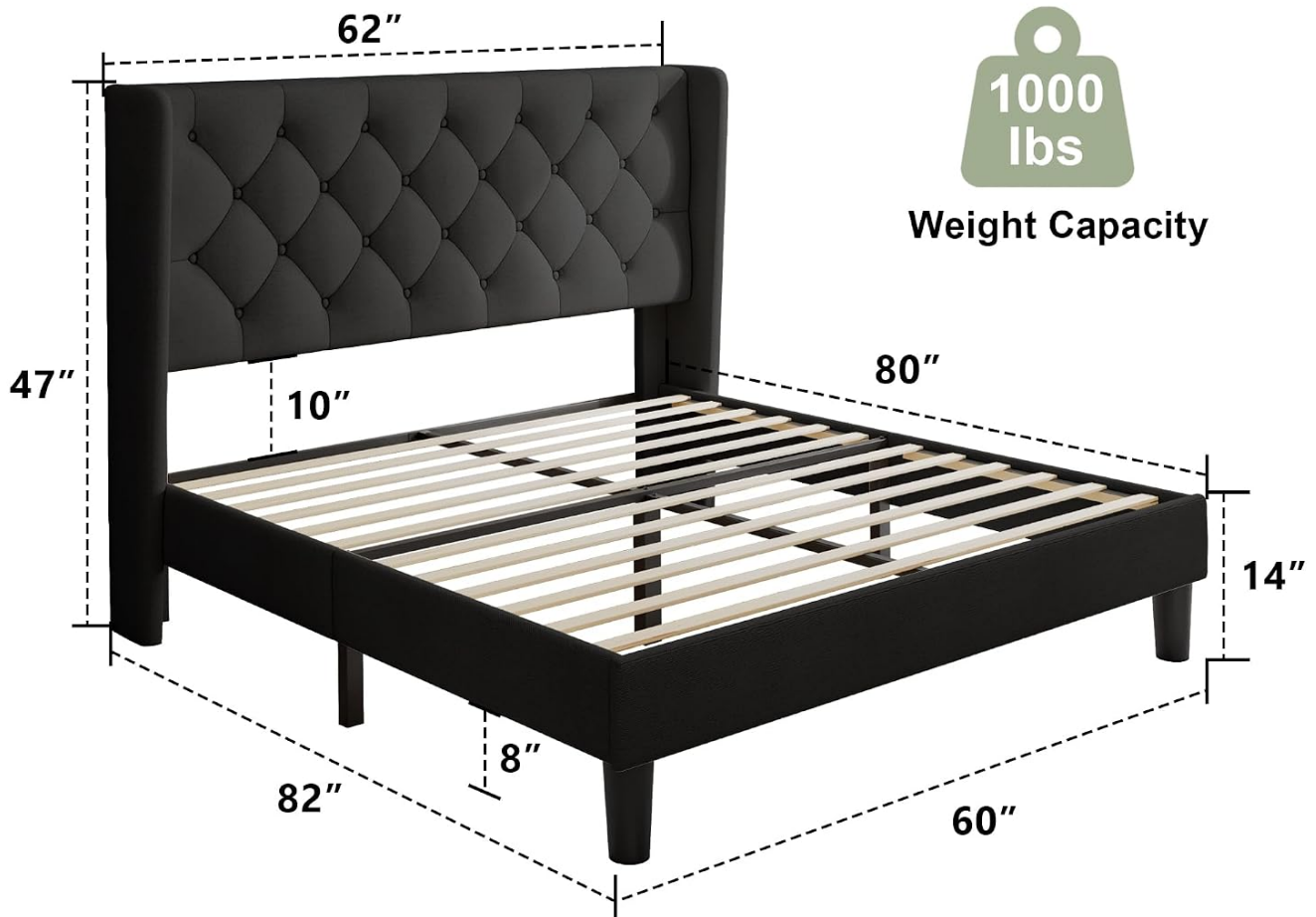
Image: Dimensional diagram for the Queen size bed frame, including overall length, width, headboard height, and the 1000 lbs weight capacity.
