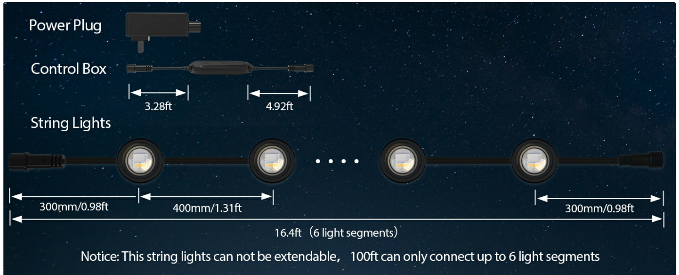
Image: Diagram of included components for APPECK Permanent Outdoor Lights C5109-C.
