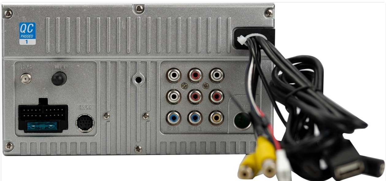
Figure 3.2: Rear panel connections of the CAR714MW.
