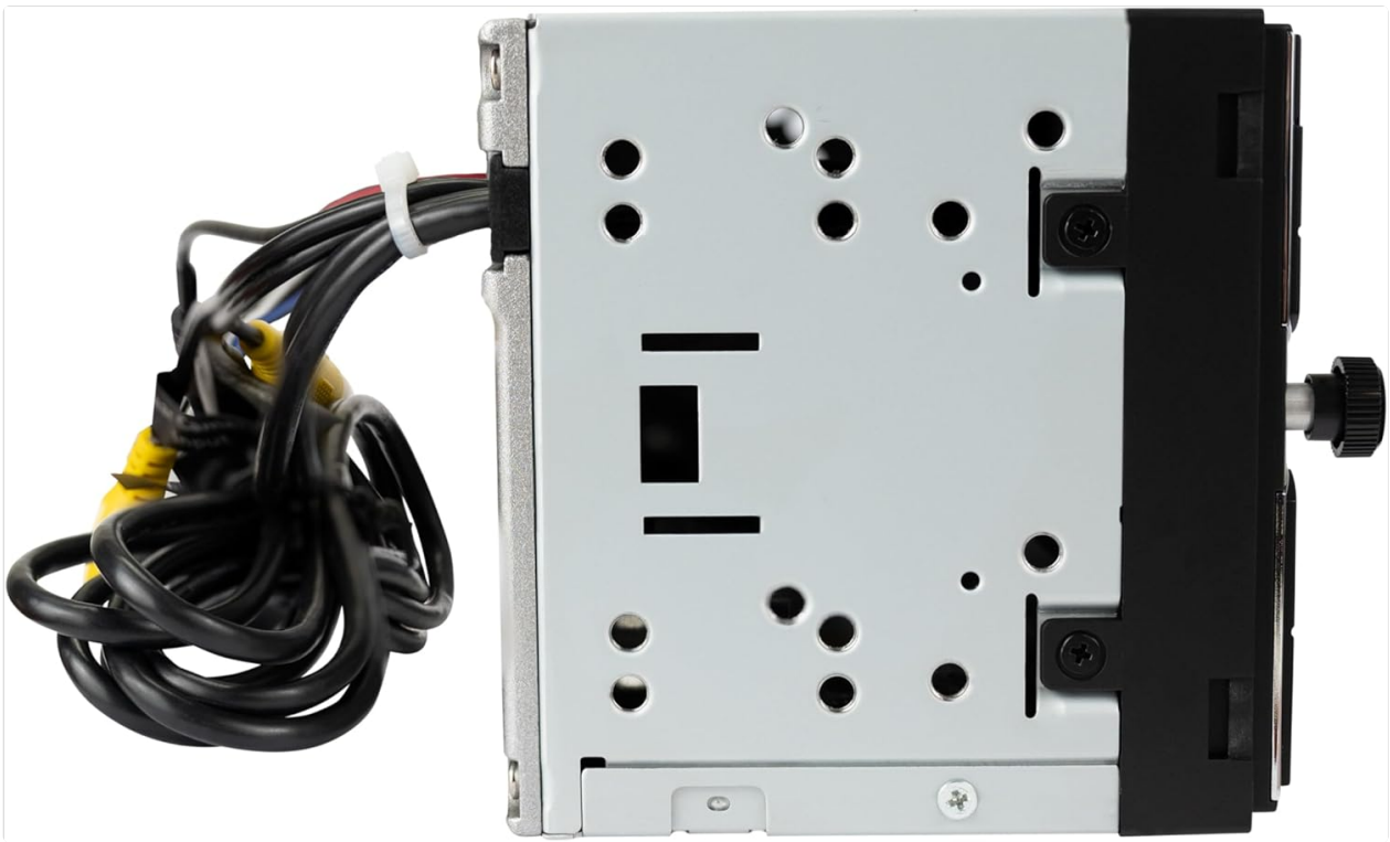
Figure 3.1: Side view of the CAR714MW unit, illustrating mounting points.
