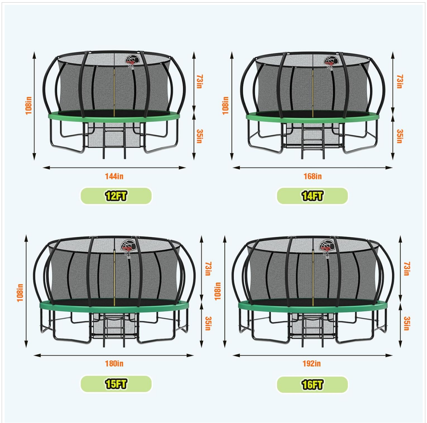
Figure 3.1: Trampoline dimensions overview.
