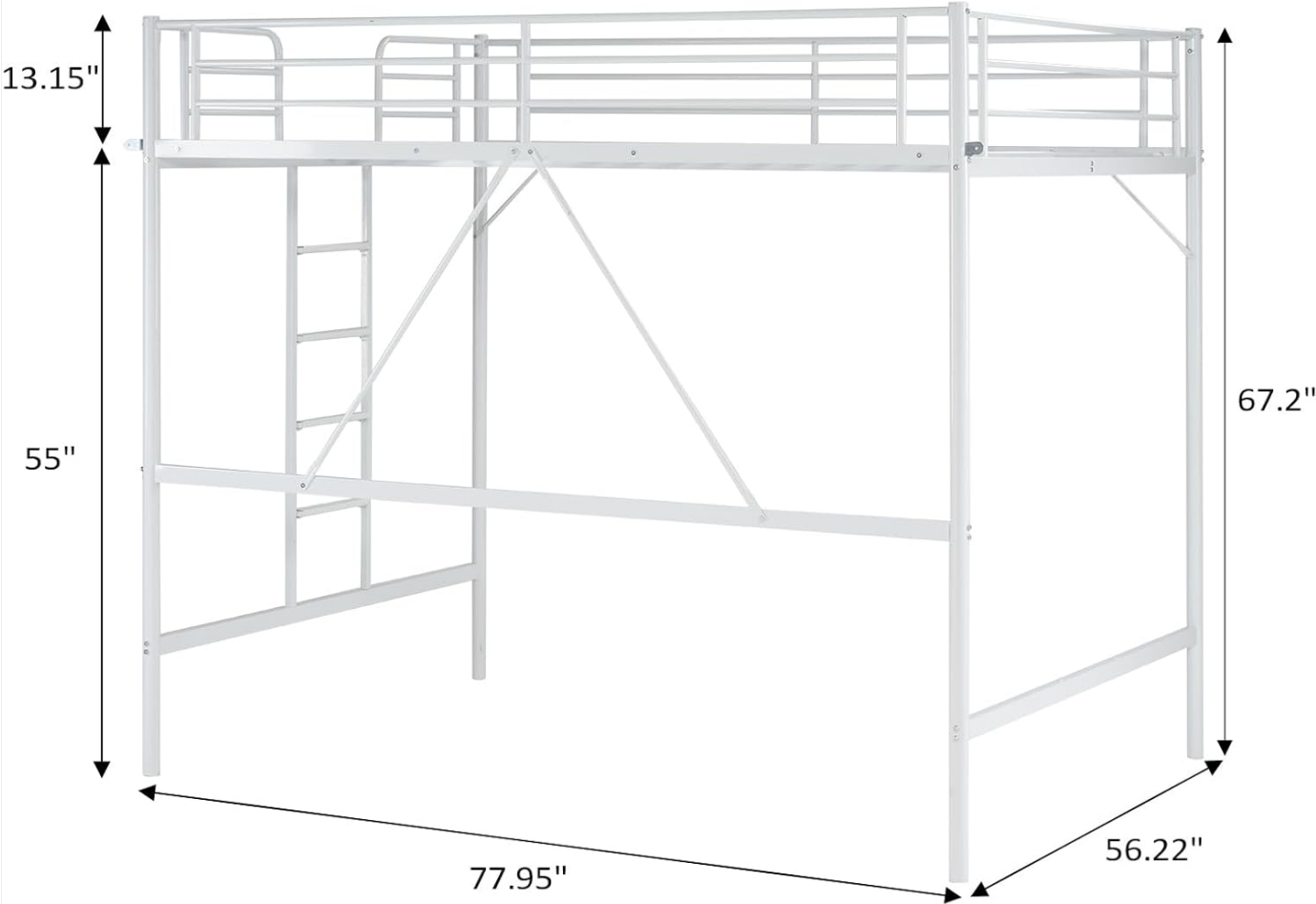
Figure 7: Product dimensions diagram.
