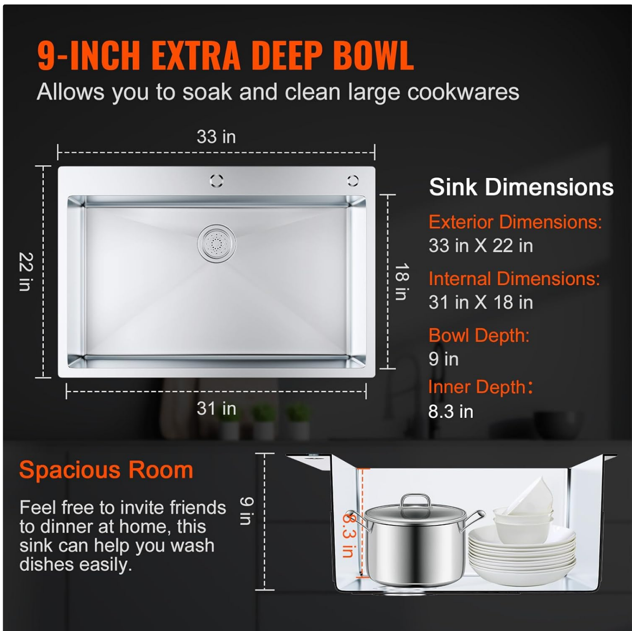
Figure 2.1: Sink Dimensions for Installation.
