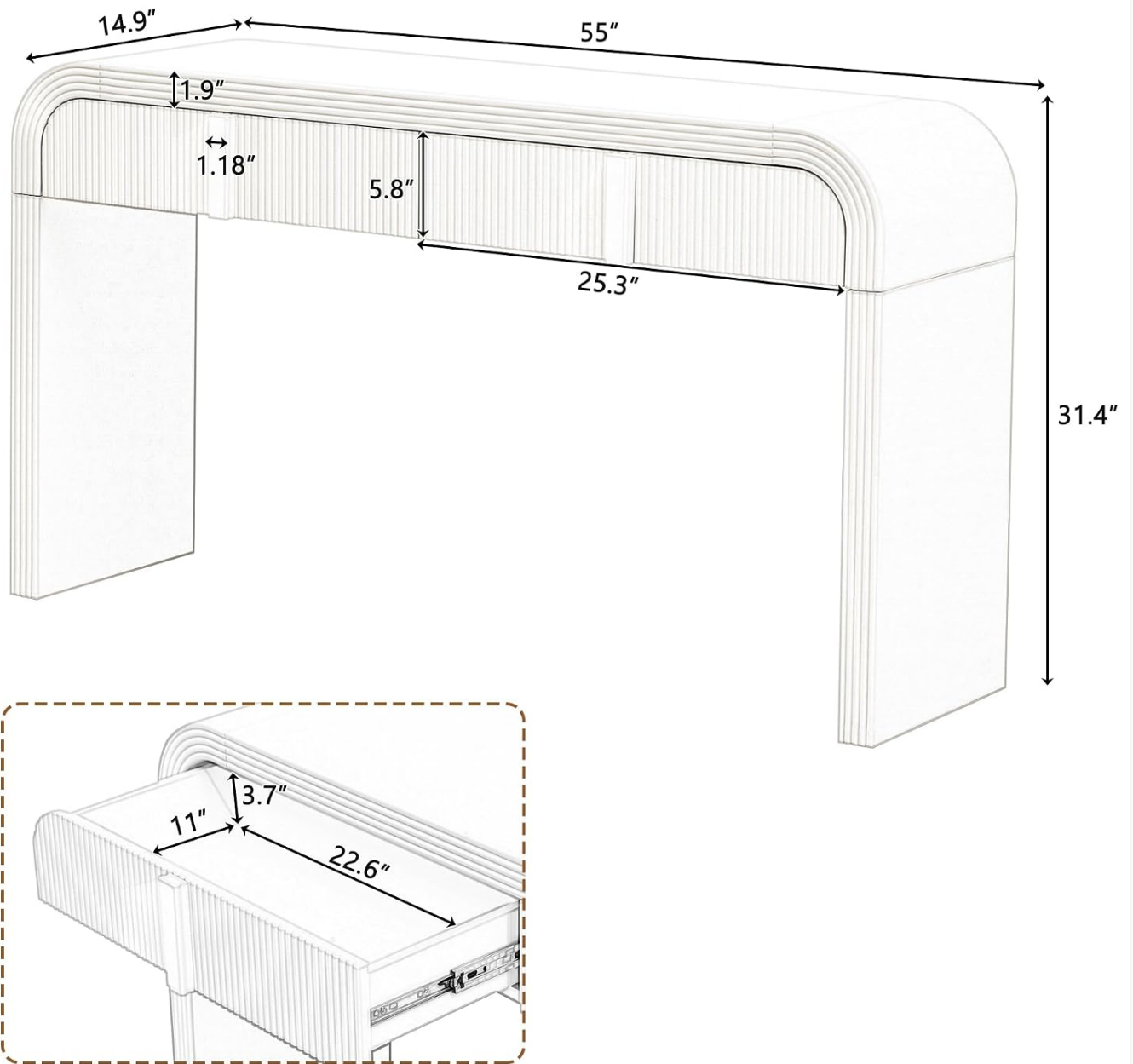
Image: A detailed diagram illustrating the overall dimensions of the console table (55"L x 14.9"W x 31.4"H) and the interior dimensions of its drawers (22.6"W x 11"D x 3.7"H).
