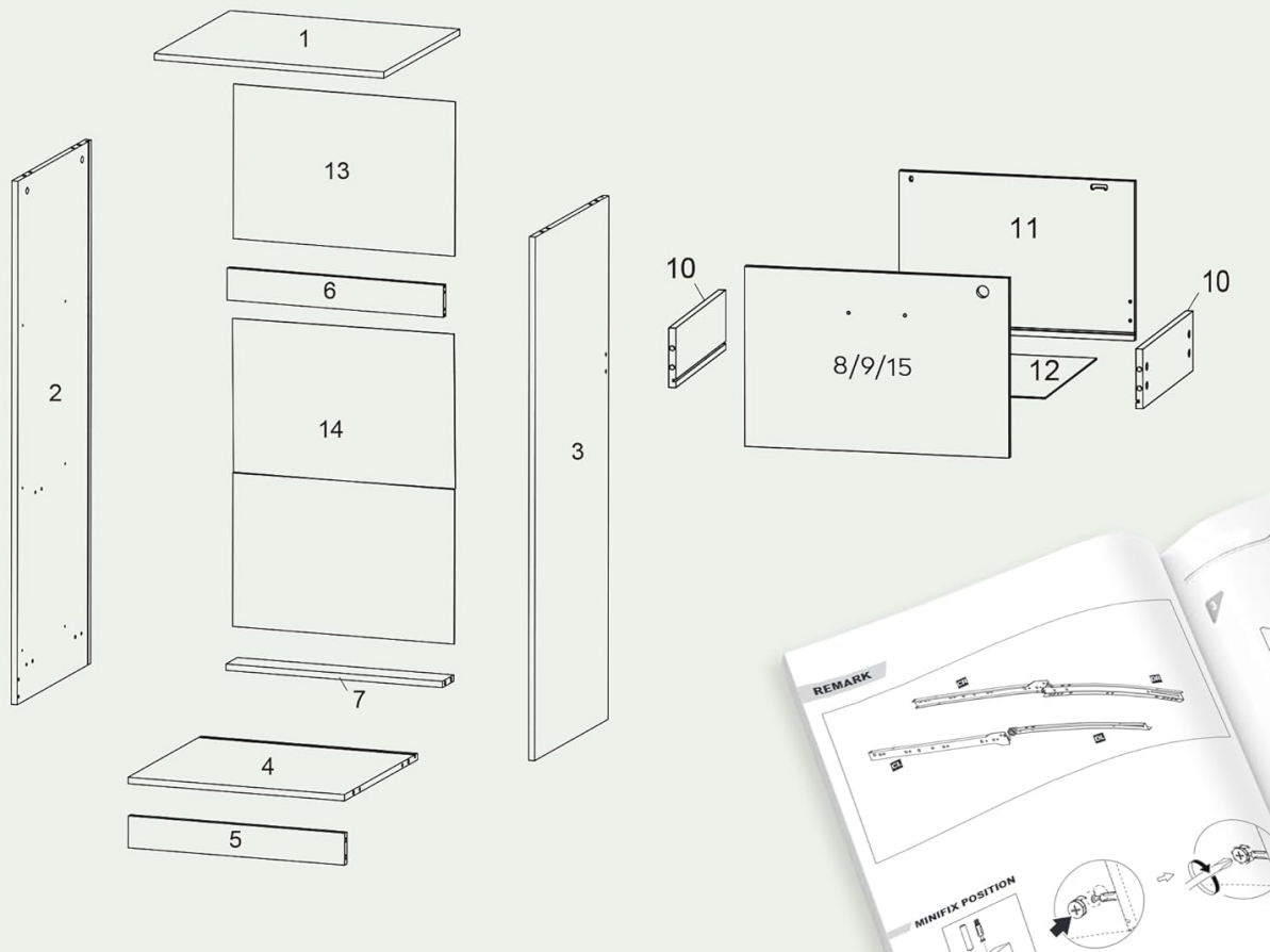
Image: An exploded diagram illustrating the labeled parts and assembly steps for the file cabinet.
