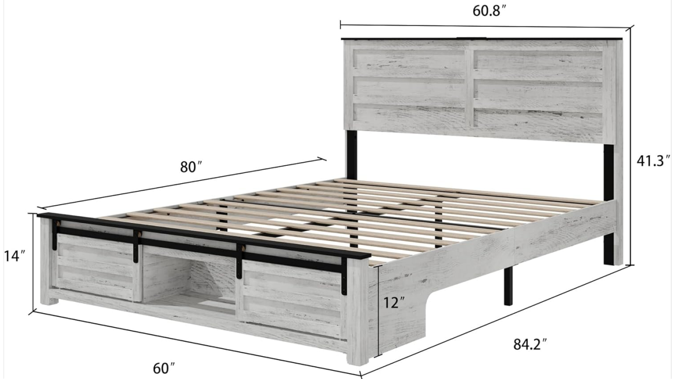
Figure 5: Detailed dimensions of the Queen Size Bed Frame.
