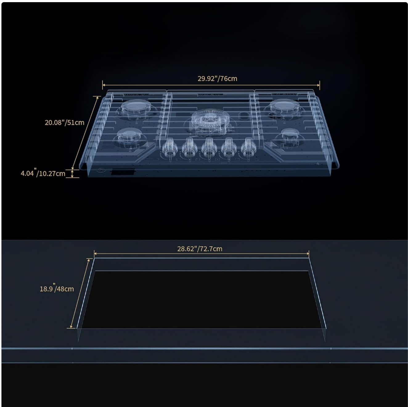
Figure 3.1: Product and cutout dimensions for the Empava 30-inch gas cooktop.
