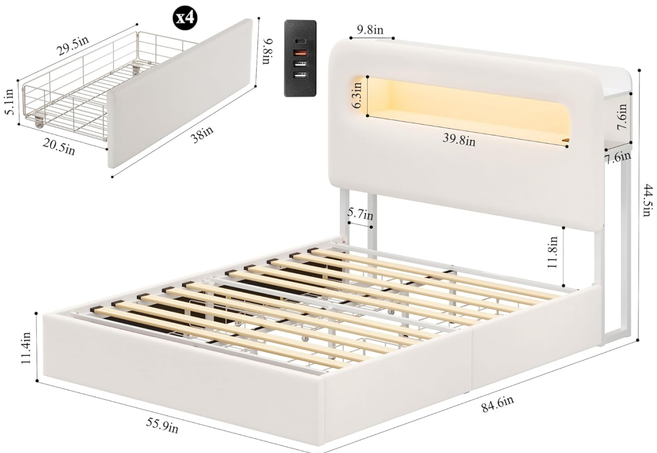
Figure 2: Overview of bed frame components and dimensions.
