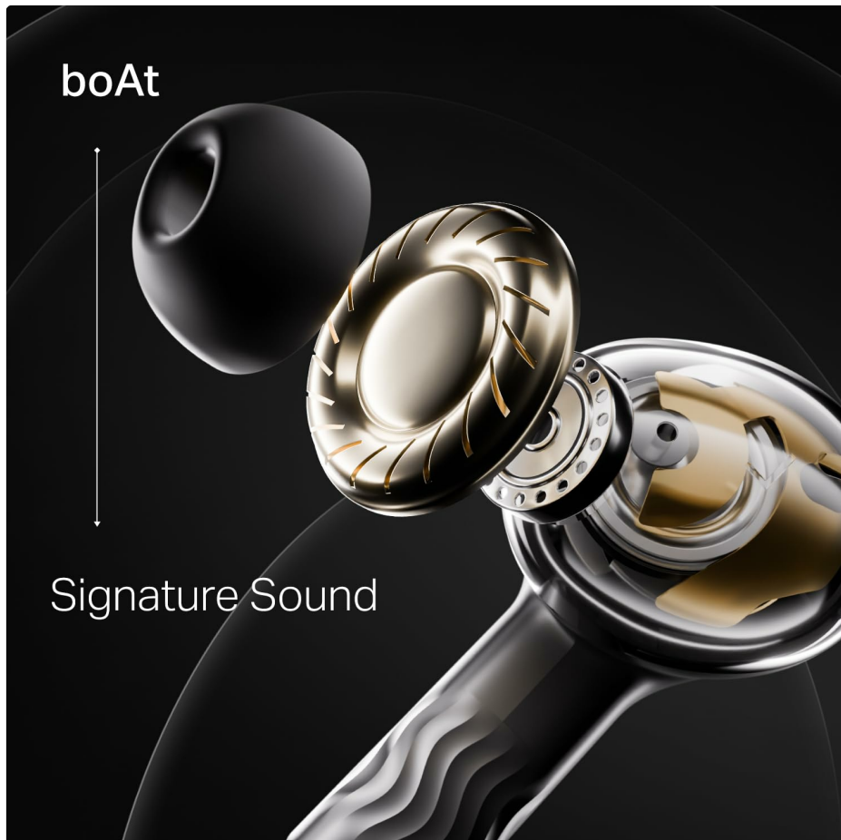
Image: An exploded view of an earbud, detailing its internal components responsible for delivering the boAt Signature Sound.
