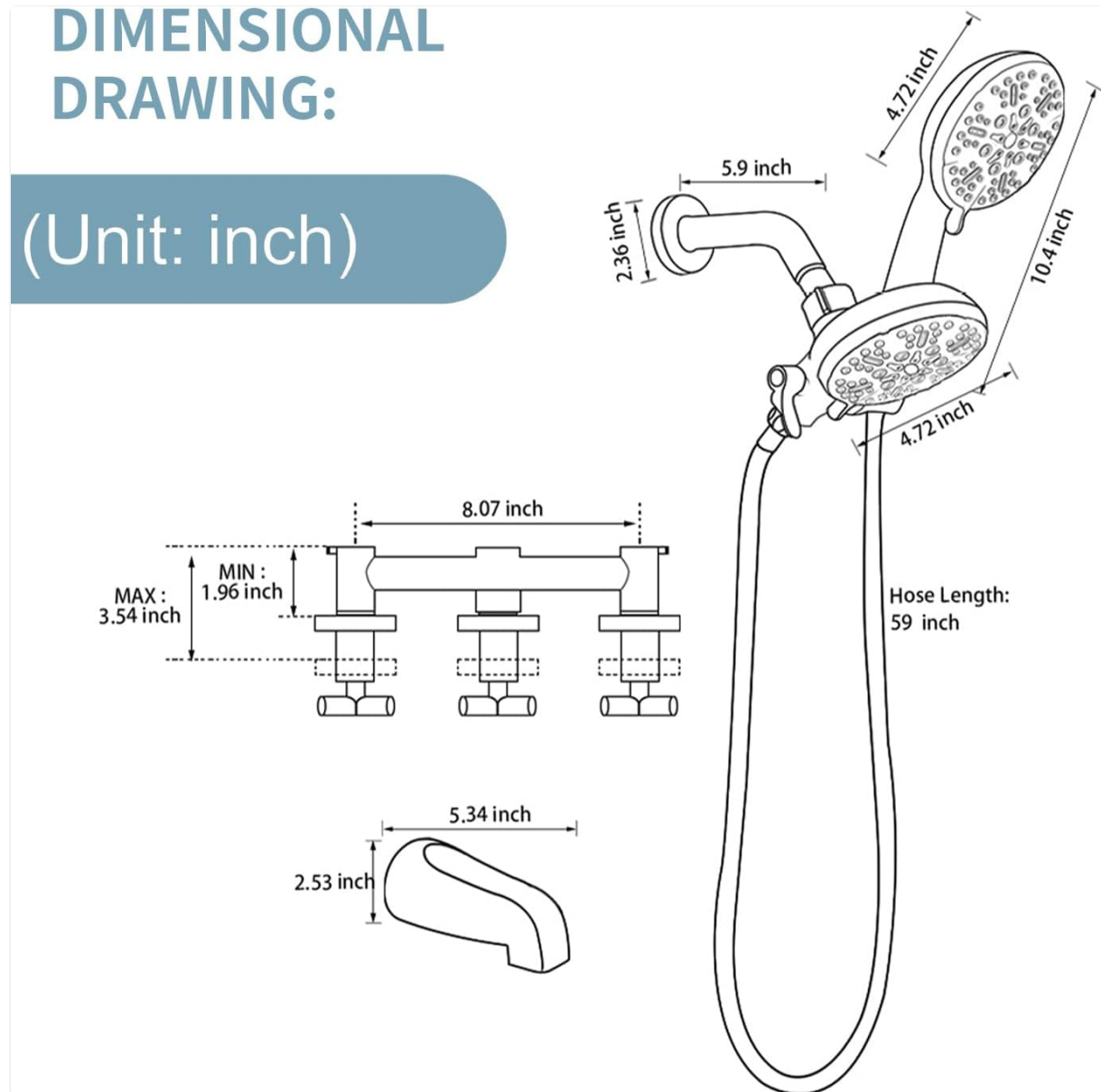
Image 4.1: Dimensional drawing showing key measurements for installation, including hose length (59 inches) and shower head dimensions.
