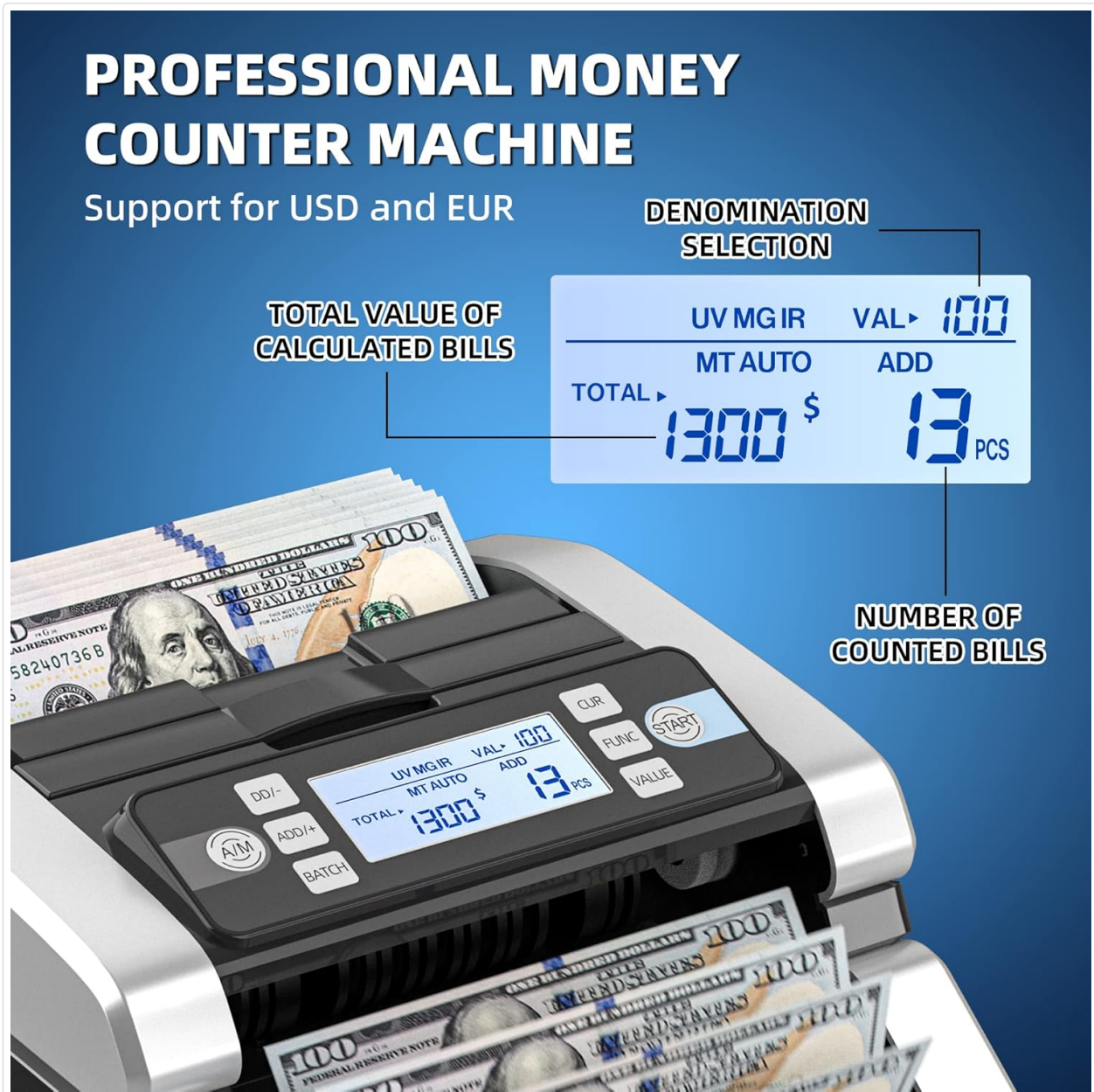
Image: A detailed view of the control panel and LCD display, illustrating the 'TOTAL' value of calculated bills and the 'PCS' (number of counted bills), along with indicators for UV, MG, IR, MT, and AUTO detection modes. Denomination selection is also shown.
