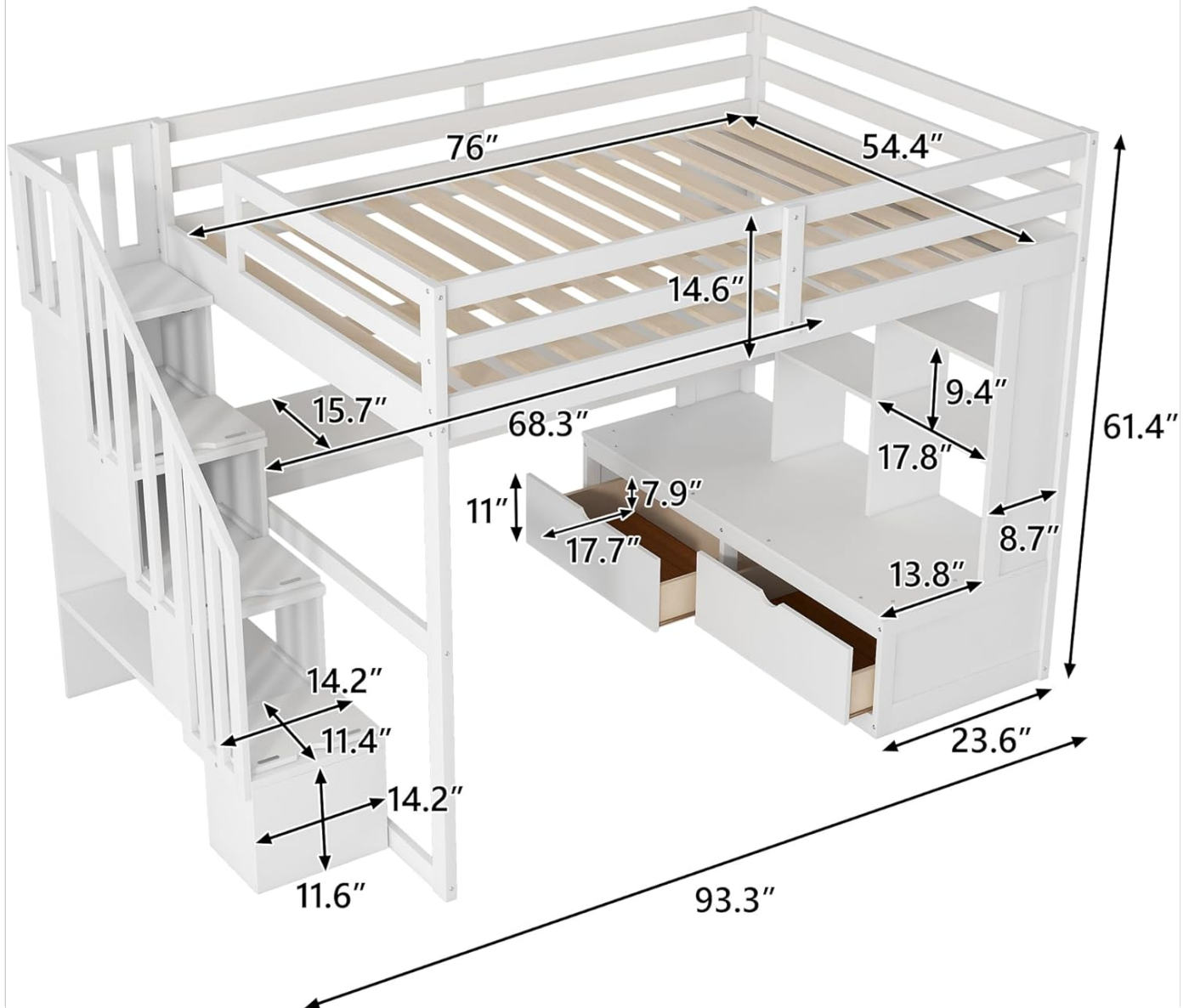
Image: Dimensional diagram of the Merax Full Size Loft Bed, illustrating overall and component measurements.
