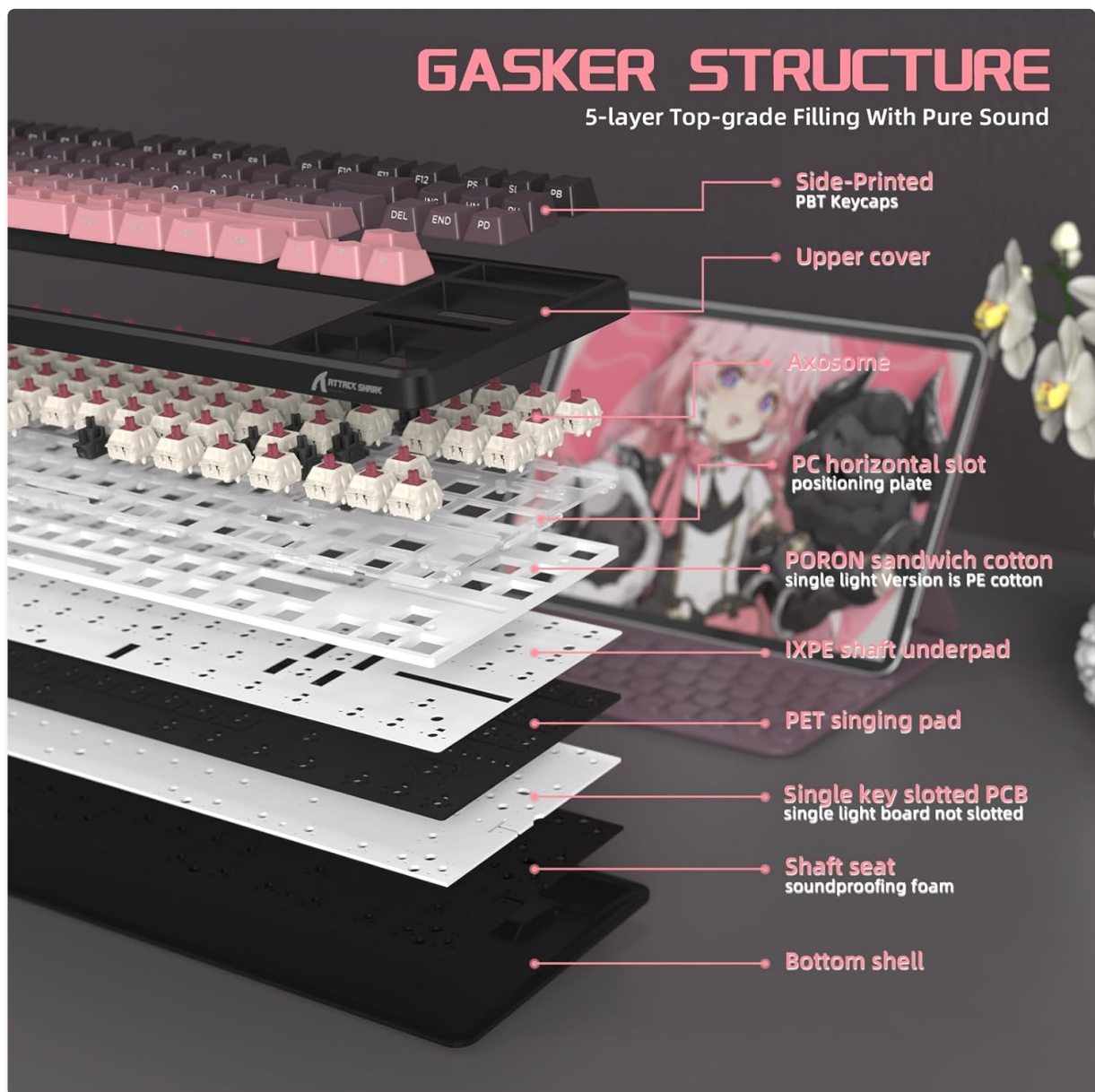
Figure 7: Exploded view of the keyboard's gasket structure and sound-absorbing layers.
