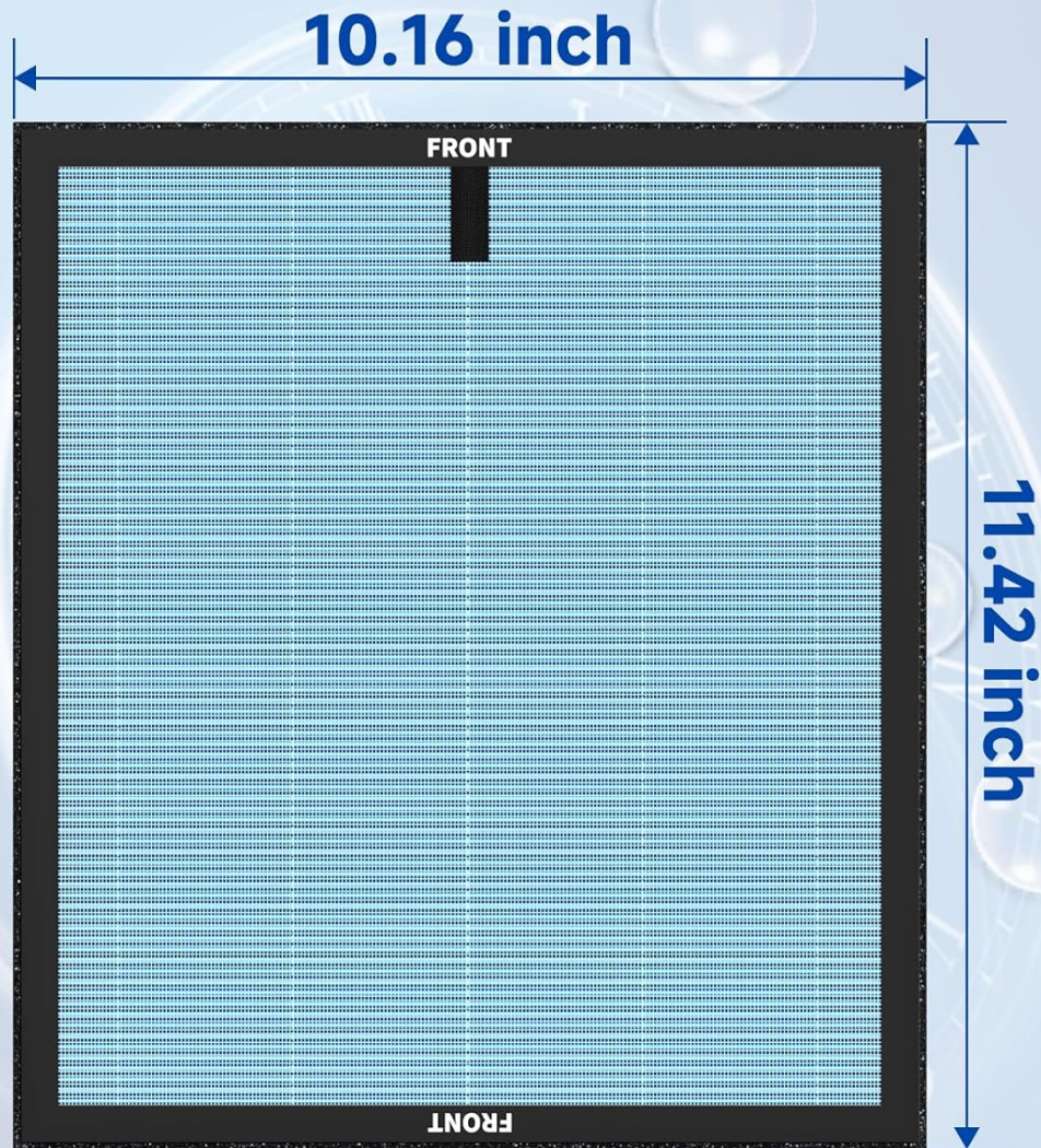
Figure 4: Detailed dimensions of the HAP603 filter.
