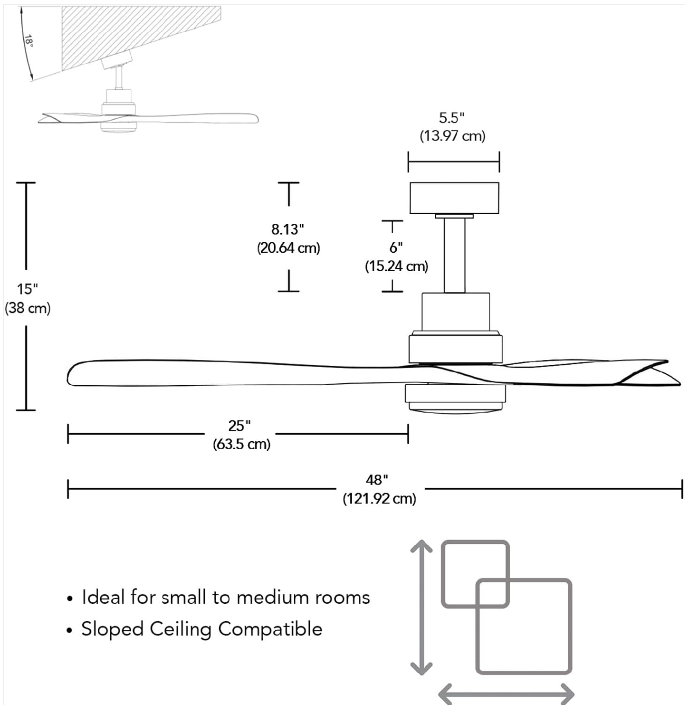
Image: A technical diagram illustrating the dimensions of the ceiling fan and its compatibility with sloped ceilings up to 18 degrees.
