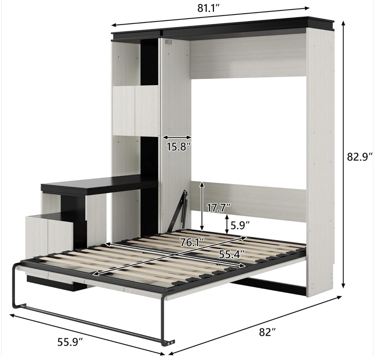
Figure 2: Overall dimensions of the Murphy Bed unit, including bed frame extended.
