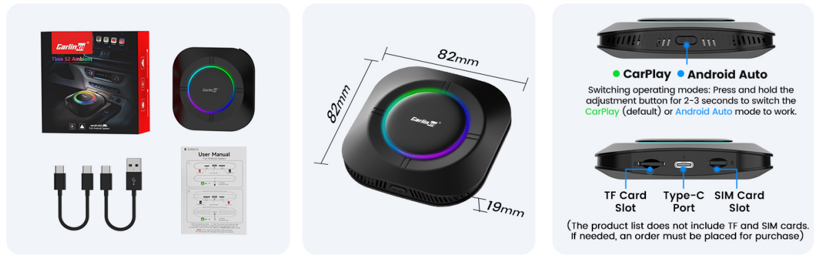
Figure 3: A detailed view of the product's dimensions, weight, and available ports including TF Card Slot, Type-C Port (Power Supply), and Nano SIM Card Slot.
