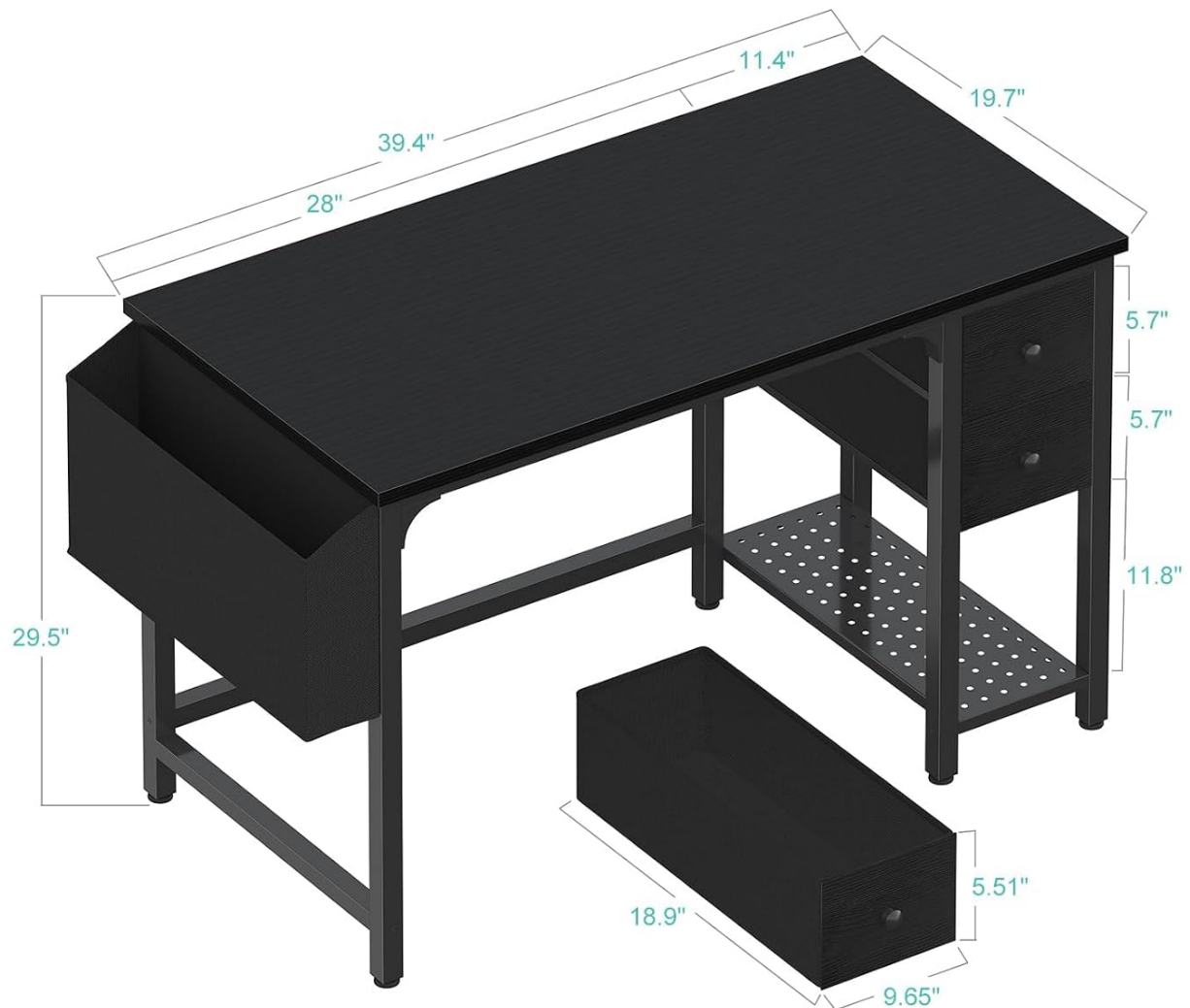
Figure 1: Product Dimensions. This diagram illustrates the overall dimensions of the desk, including width, depth, and height, along with measurements for the drawers and side storage.
