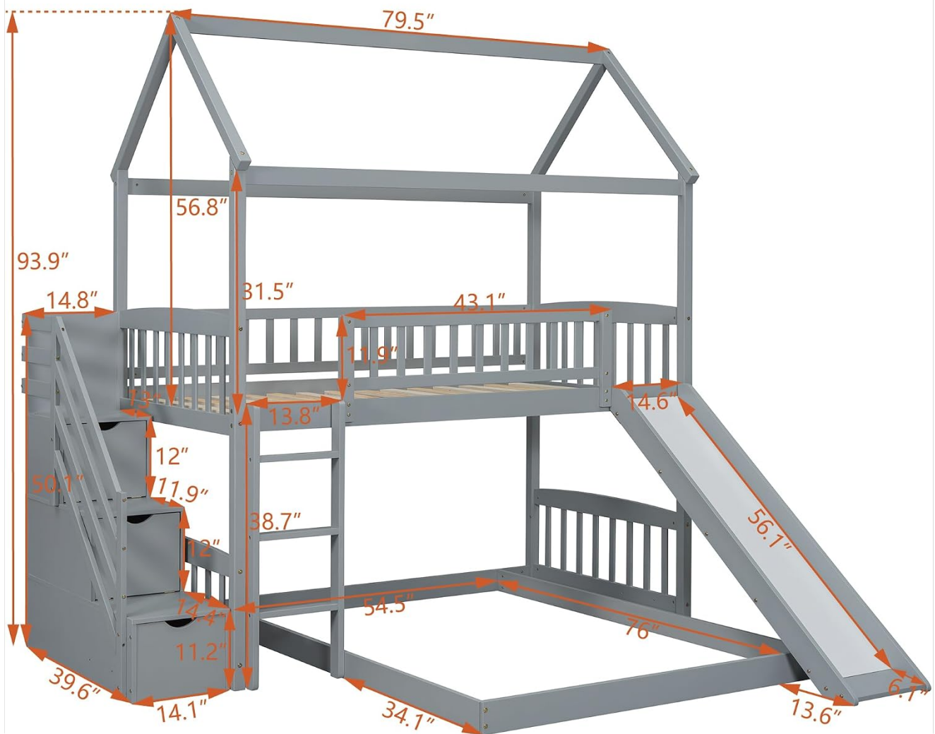
Image 4.1: Dimensional drawing of the bunk bed, showing overall length, width, height, and specific measurements for the slide, stairs, and bed levels.
