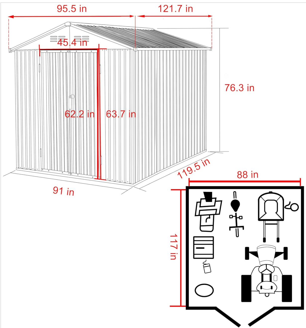
Image 8.1: Dimensional drawing of the VEIKOU 8x10FT storage shed.
