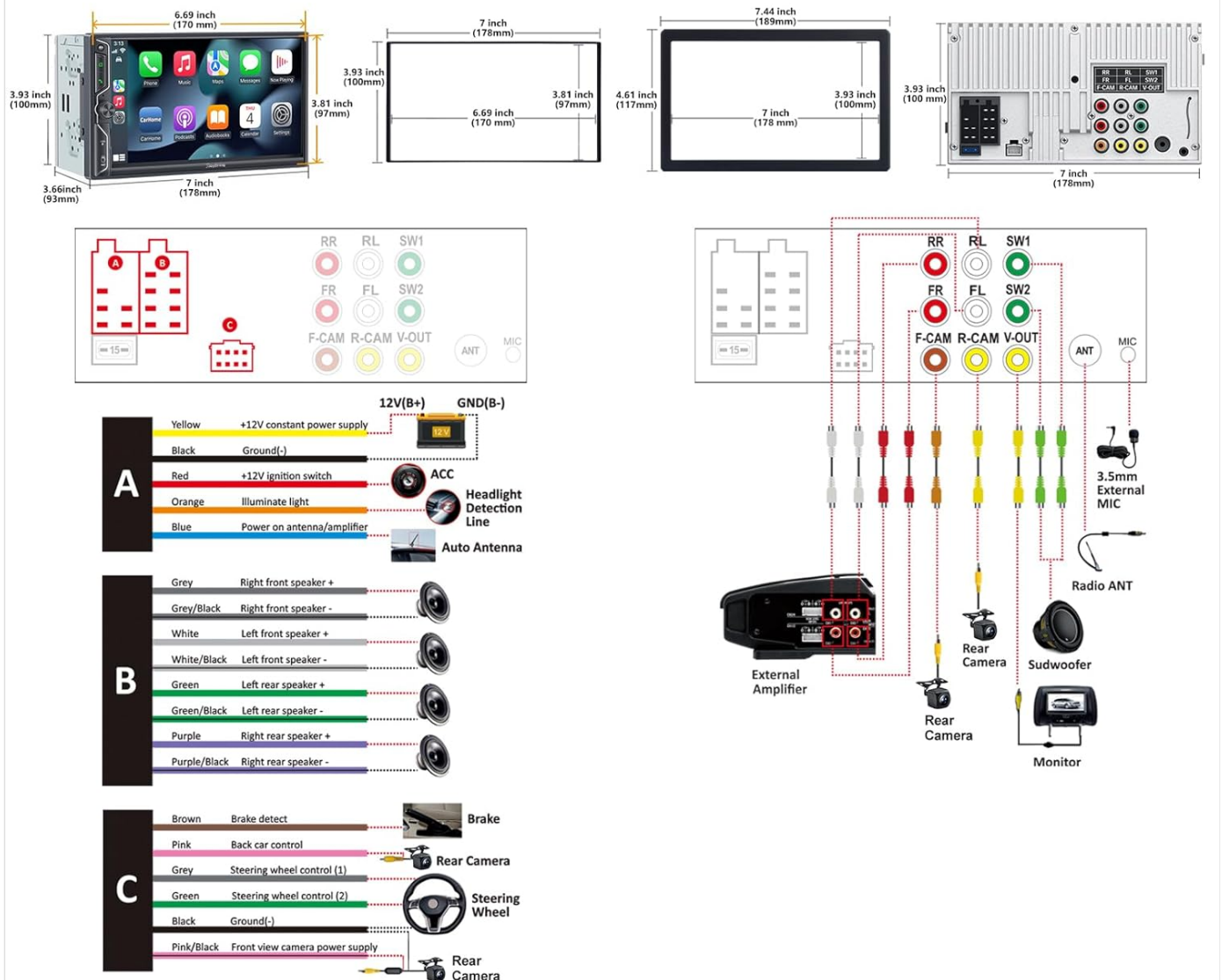
Image: Detailed diagram showing the dimensions of the car stereo and various wiring connections for power, speakers, cameras, and external amplifiers. It also highlights the mounting holes for installation.
