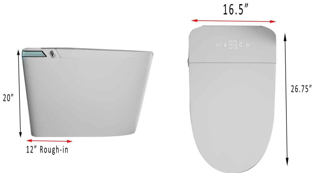
Detailed diagram showing the product dimensions for installation planning.
