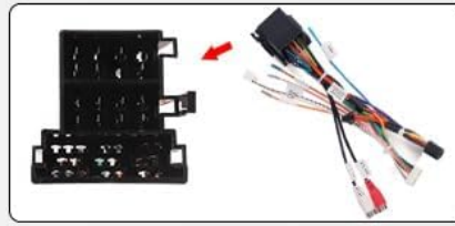
ISO power harness
