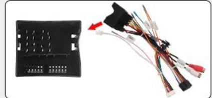
Quadlock power harness
