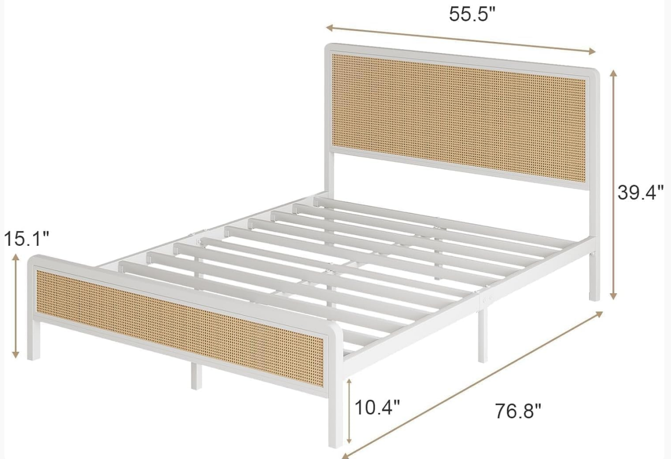
Image 7.1: Detailed dimensions of the Full Rattan Bed Frame, including length, width, height, and under-bed clearance.
