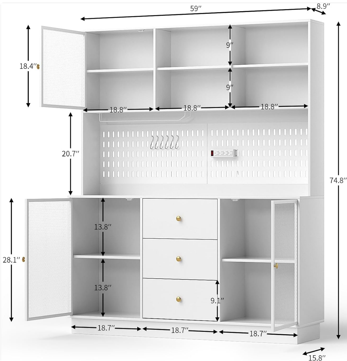
Image: A diagram illustrating the precise dimensions of the VOWNER Large Kitchen Hutch Cabinet, including width, depth, and height, along with internal shelf and compartment measurements.
