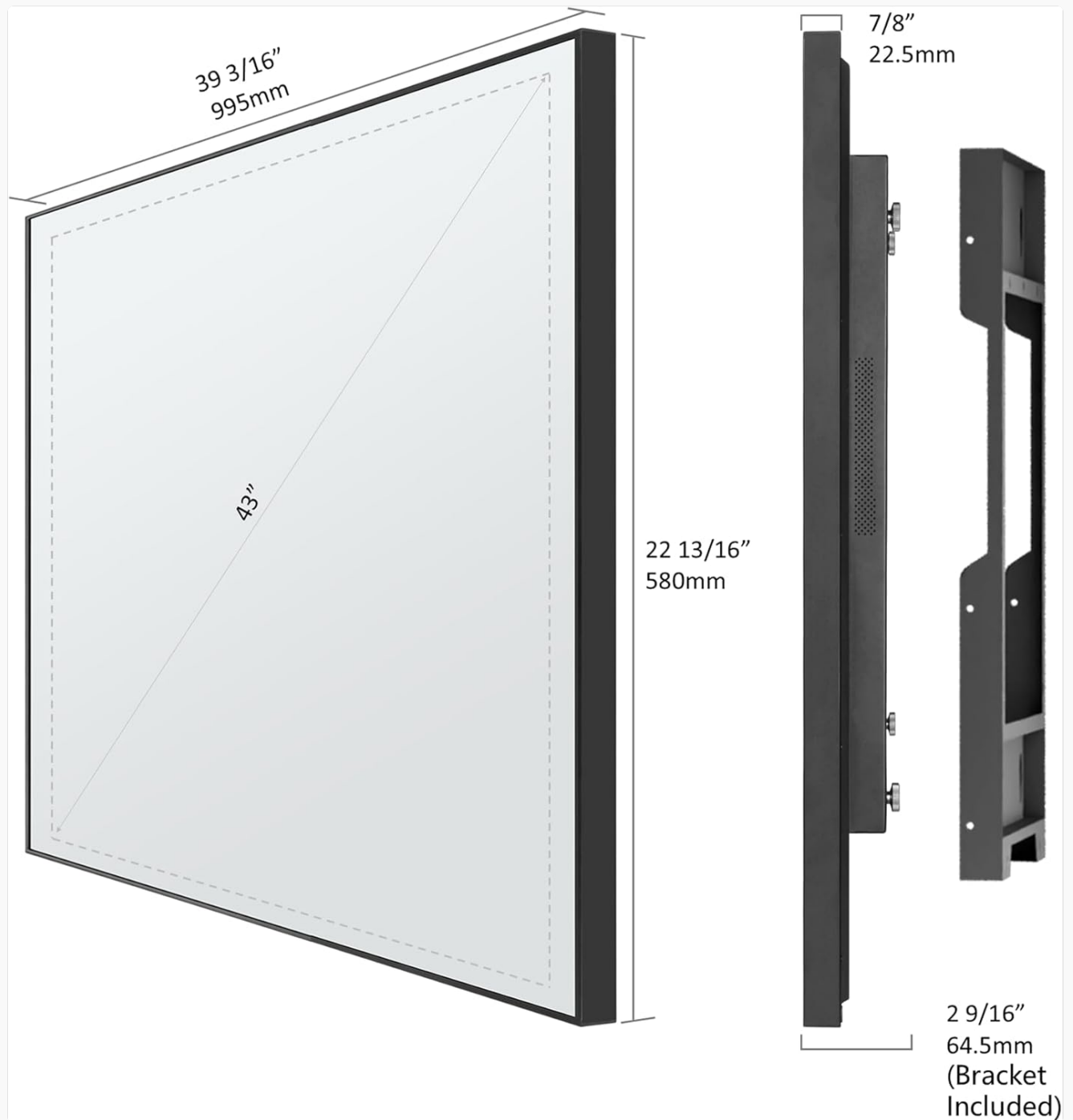
Figure 4.2: Product dimensions with bracket.
