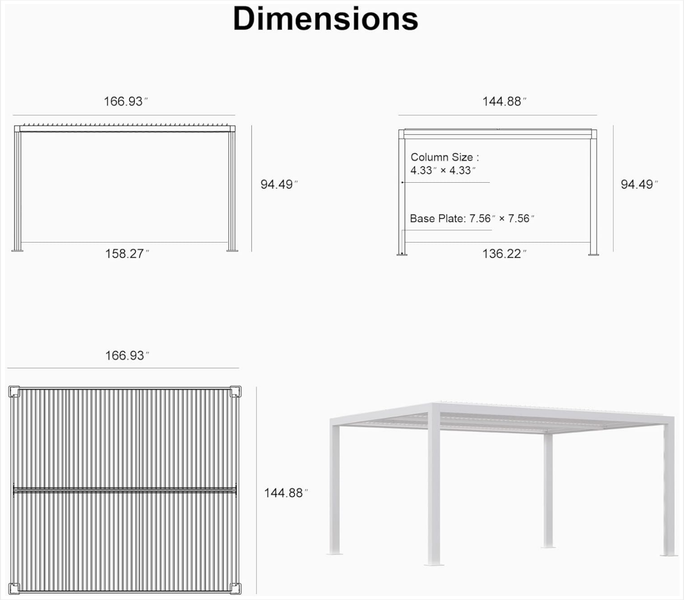
Image: Detailed diagram showing the overall dimensions of the pergola, including length, width, height, column size, and base plate size. This provides essential measurements for planning and installation.
