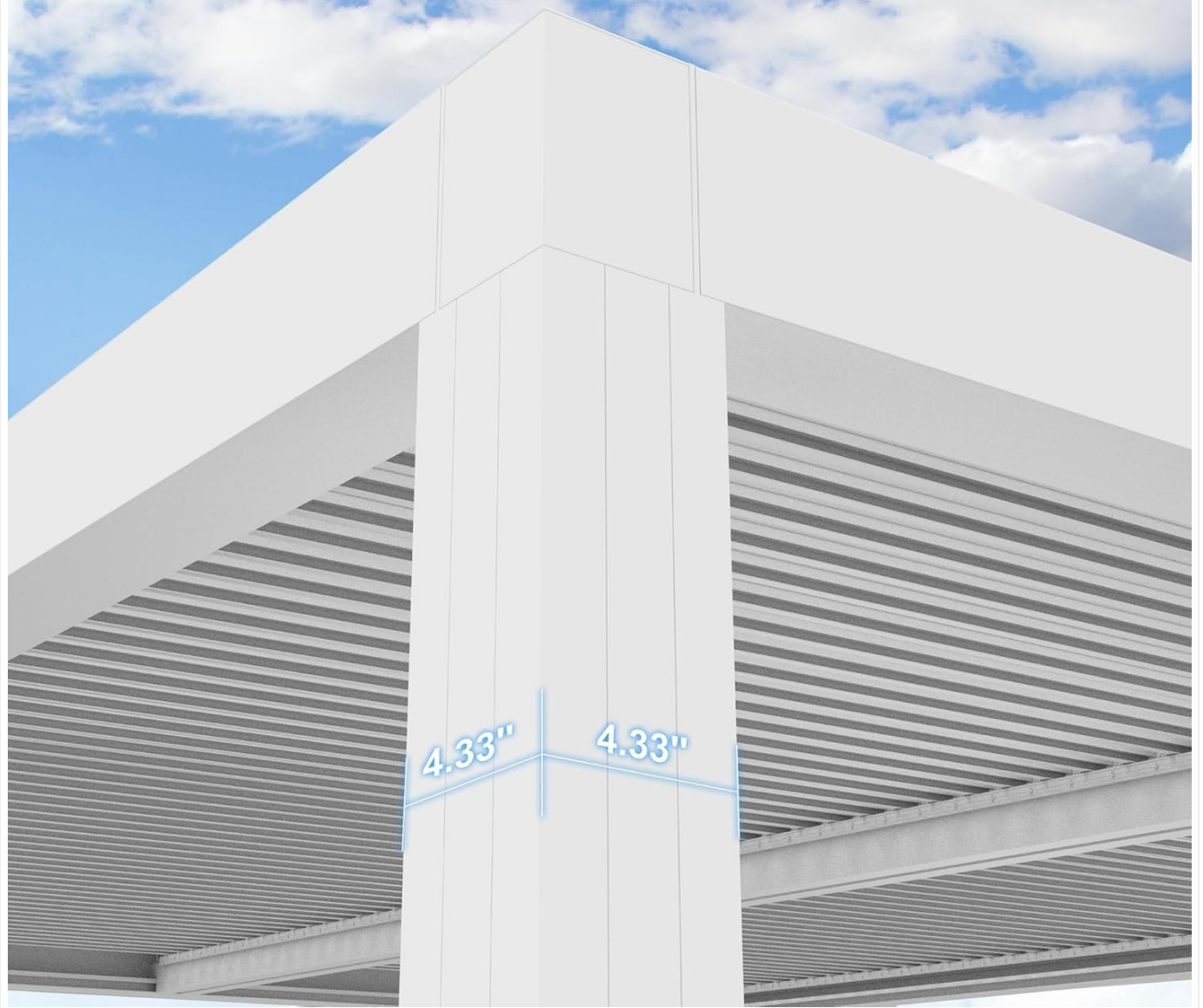
Image: Close-up of the aluminum frame, highlighting the dimensions of the columns (4.33" x 4.33") and emphasizing its corrosion-resistant, lighter, sturdier, and longer-lasting properties.
