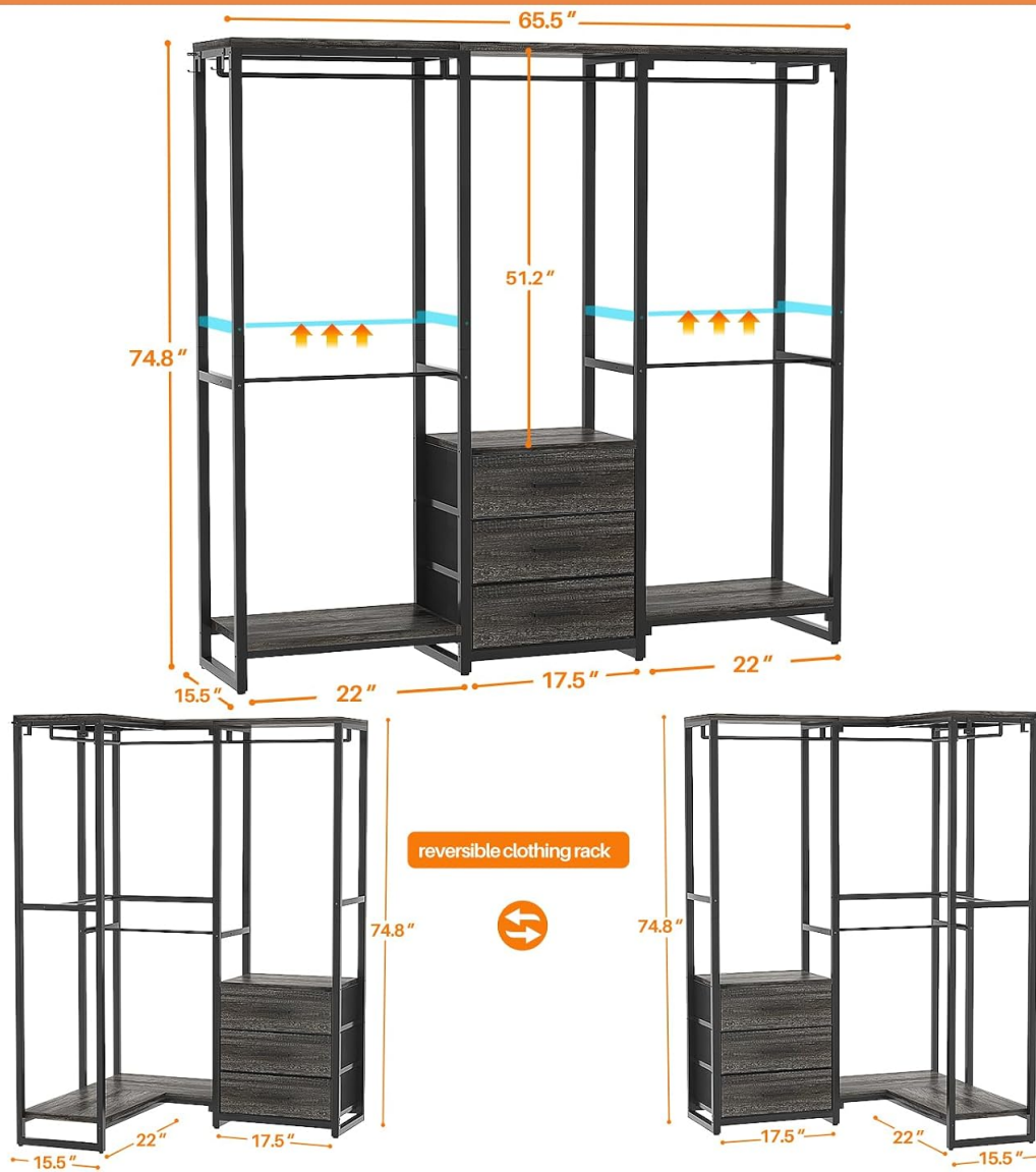
Image: Technical diagram illustrating the dimensions and two primary assembly configurations (L-shape and straight-lined) of the Aheaplus Garment Rack.
