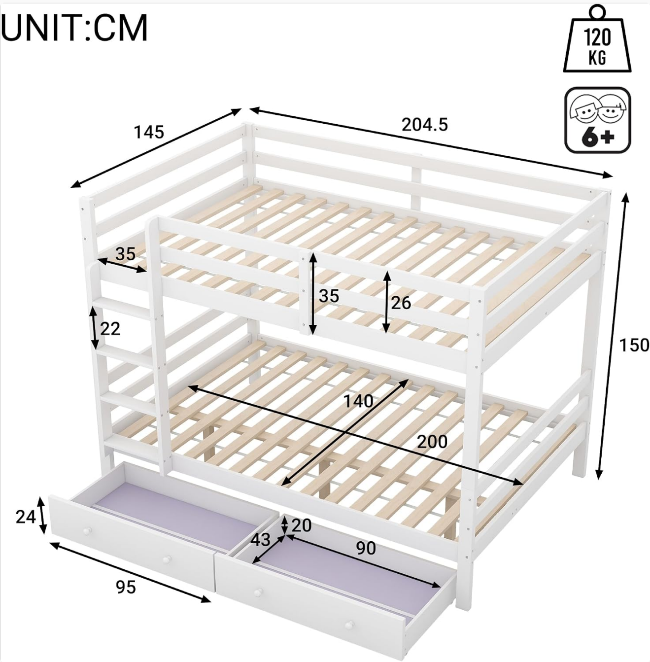
Figure 6: Detailed diagram illustrating the dimensions of the Moimhear 140x200cm Bunk Bed in centimeters, including overall length, width, height, and internal bed dimensions, as well as drawer and ladder measurements. It also indicates a 120kg weight capacity and suitability for ages 6+.
