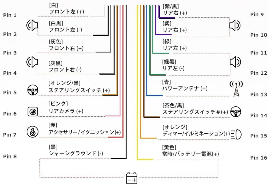
Image: Detailed wiring diagram for the ATOTO S8 Ultra, showing connections for power, speakers, cameras, and other peripherals.
