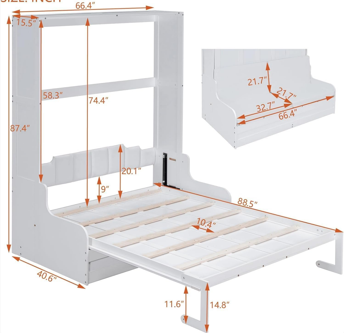
Image 6.1: Dimensional diagram illustrating the key measurements of the Murphy bed and sofa unit.
