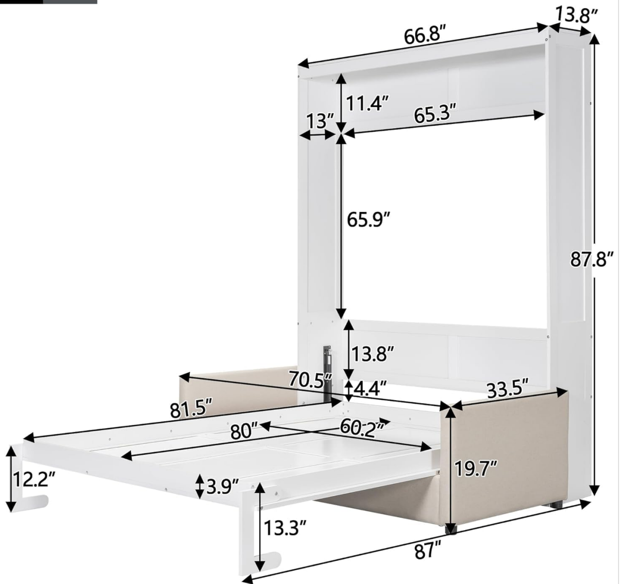
Figure 1: Dimension diagram of the MERITLINE Queen Murphy Bed with Couch, illustrating key measurements for planning and assembly.
