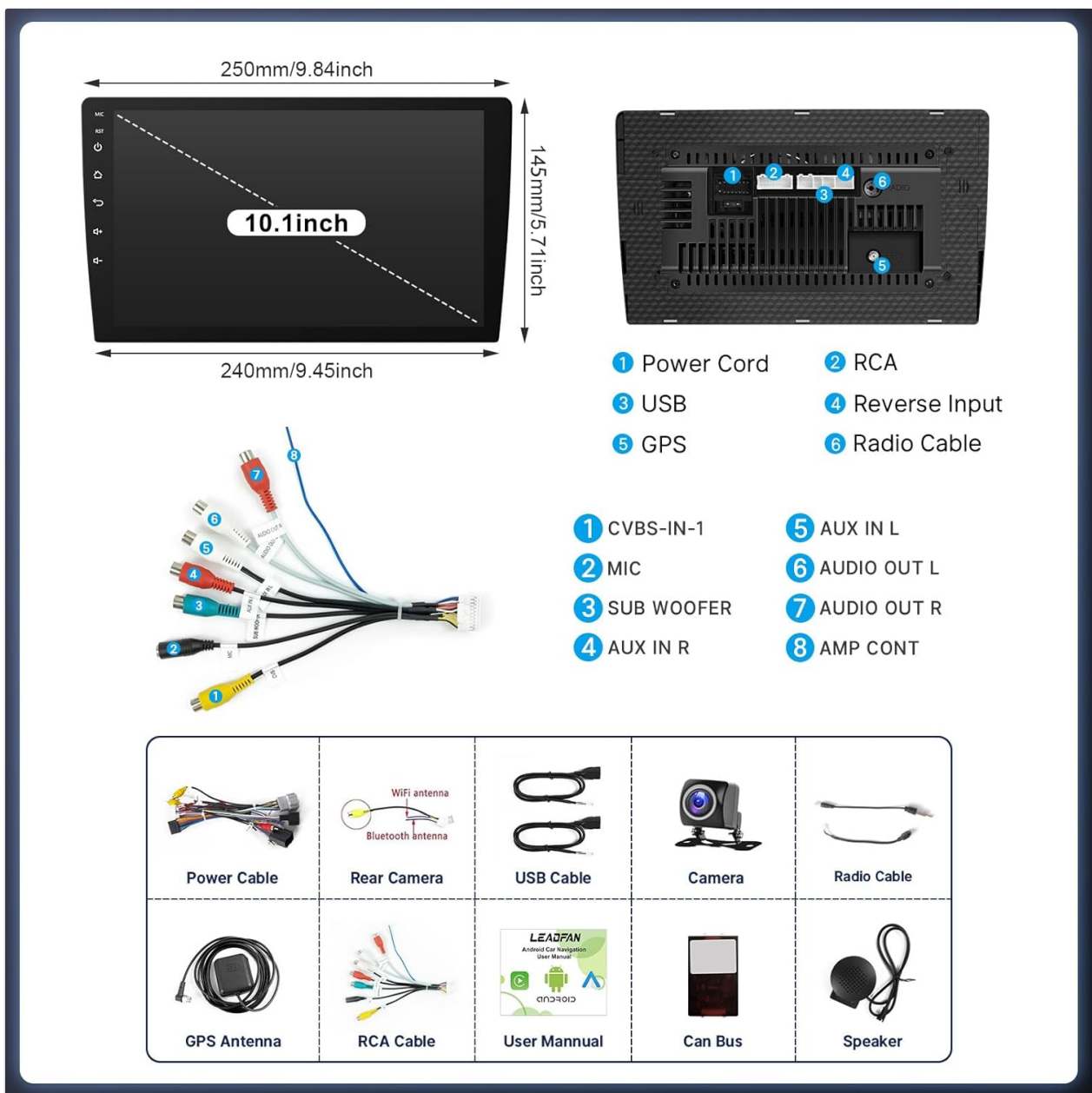
Image: Detailed diagram of the head unit's dimensions, rear connections, and a comprehensive list of all components included in the package.
