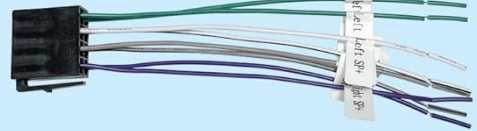
Wire Harness A
