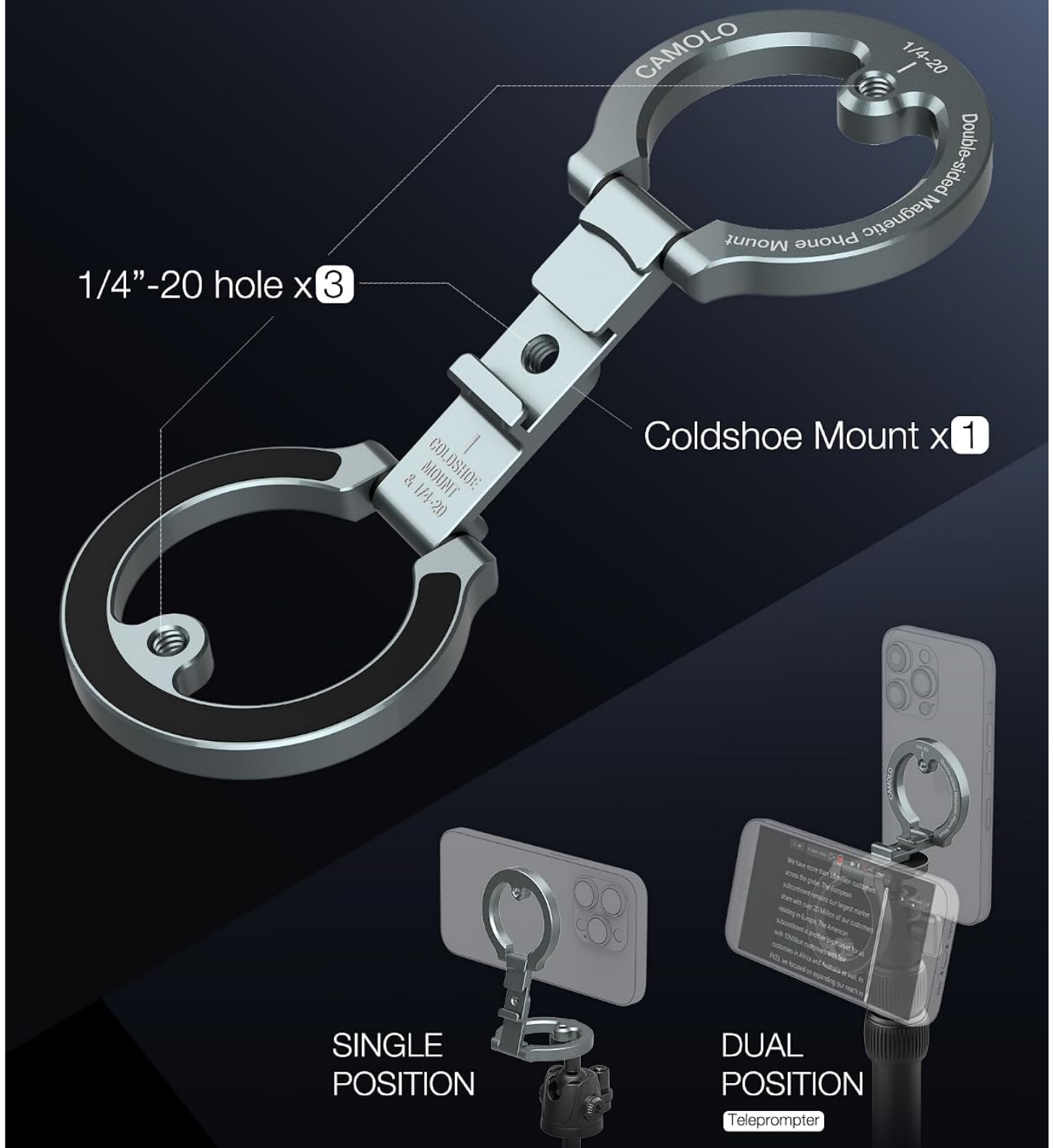
Figure 4.2: The holder features multiple 1/4"-20 screw holes and a cold shoe mount for attaching to tripods and other photographic accessories.
