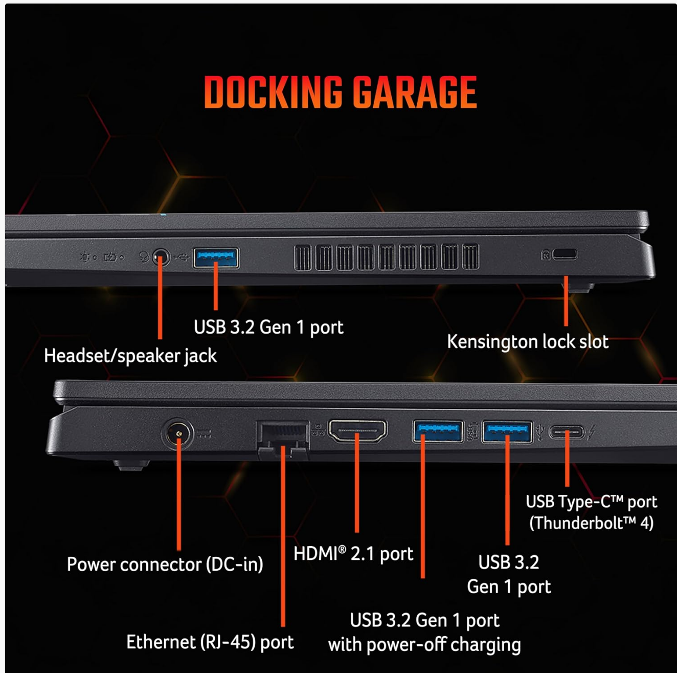
Figure 7: Overview of the laptop's various input/output ports.
